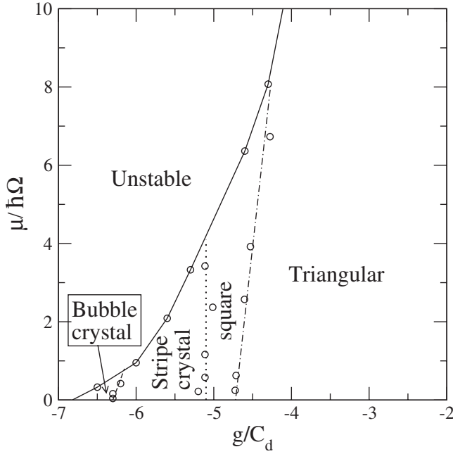
FIG. 1. The phase diagram for a trap asymmetry a_{\parallel}/\ell=0.4 . The horizontal axis gives the ratio of the contact to dipolar interactions and the vertical axis is the chemical potential (normalized to the energy corresponding to the rotation frequency \Omega of the condensate). The condensate is unstable to collapse on the left of the solid line. Marked on the figure are the regions where vortex lattices of different symmetries are the ground state of the system. The lines are fits to numerical results marked by circles.
