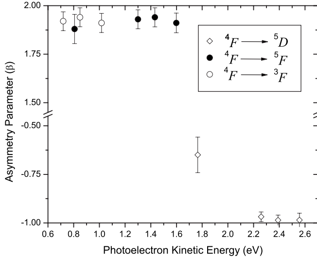
FIG. 7. A plot of asymmetry parameters versus center-of-mass photoelectron kinetic energies for all measured photon wavelengths for the 4F \rightarrow 5D ( \diamond ), 4F \rightarrow 5F ( \bullet ), and 4F \rightarrow 3F ( \circ ) \text{Fe}^- photodetachment channels. It is interesting to note that the asymmetry parameter value for the parity “unfavored” 4F \rightarrow 5D transition near 1.8 eV is not \beta = -1 , as would be expected from angular momentum transfer theory. Moreover, within experimental error bars shown to one standard deviation of the mean, the asymmetry parameters for s -electron detachment are not identically \beta = 2 , as would be expected.
