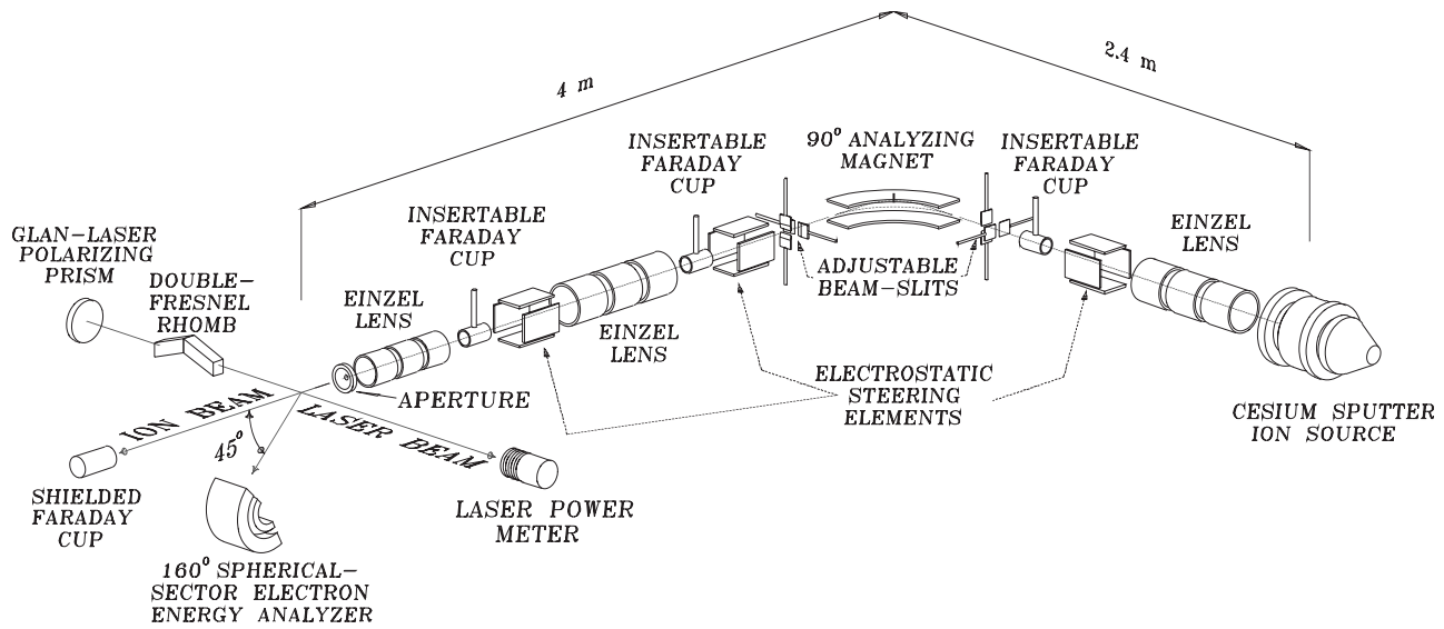
FIG. 1. Laser photodetachment electron spectroscopy (LPES) experimental apparatus.
