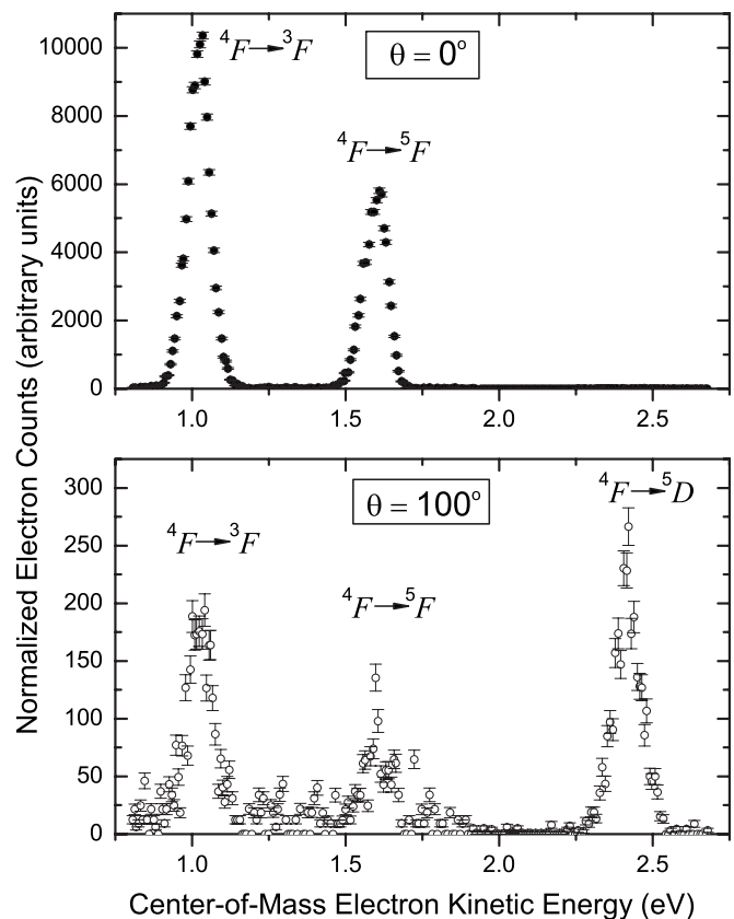
FIG. 6. Photoelectron kinetic energy spectra for the photodetachment of \text{Fe}^- at \lambda=457.9 nm and at polarization angles of \theta=0^\circ and 100^\circ .
