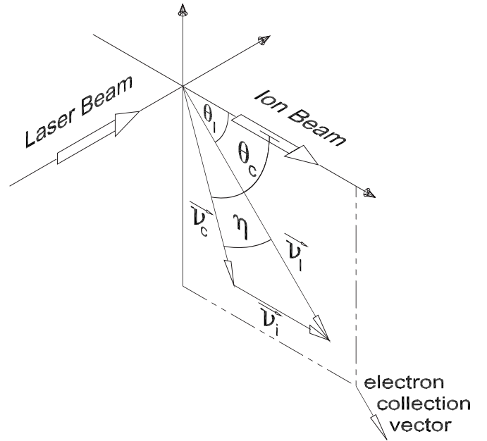
FIG. 2. Kinematic transformation diagram for ion ( \vec{v}_i ), center-of-mass photoelectron ( \vec{v}_c ), and laboratory-frame photoelectron ( \vec{v}_l ), velocity vectors.
