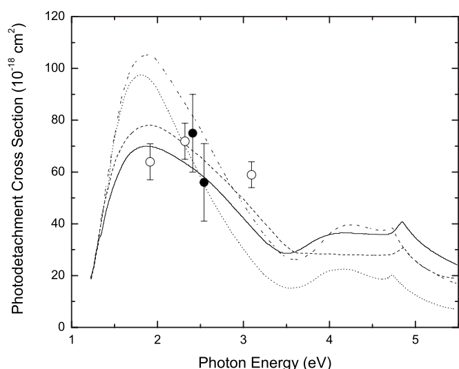
FIG. 8. A comparison of Cu^- photodetachment cross sections: The present experimental cross sections (●) are compared with the previous experimental values (○) of Balling et al. [6] and calculations of Scheibner and Hazi [2]. The curves represent two different ab initio R -matrix models in velocity and length form model B1: length form (---) and velocity form (····), and model B2: length form (- - -) and velocity form (—).
