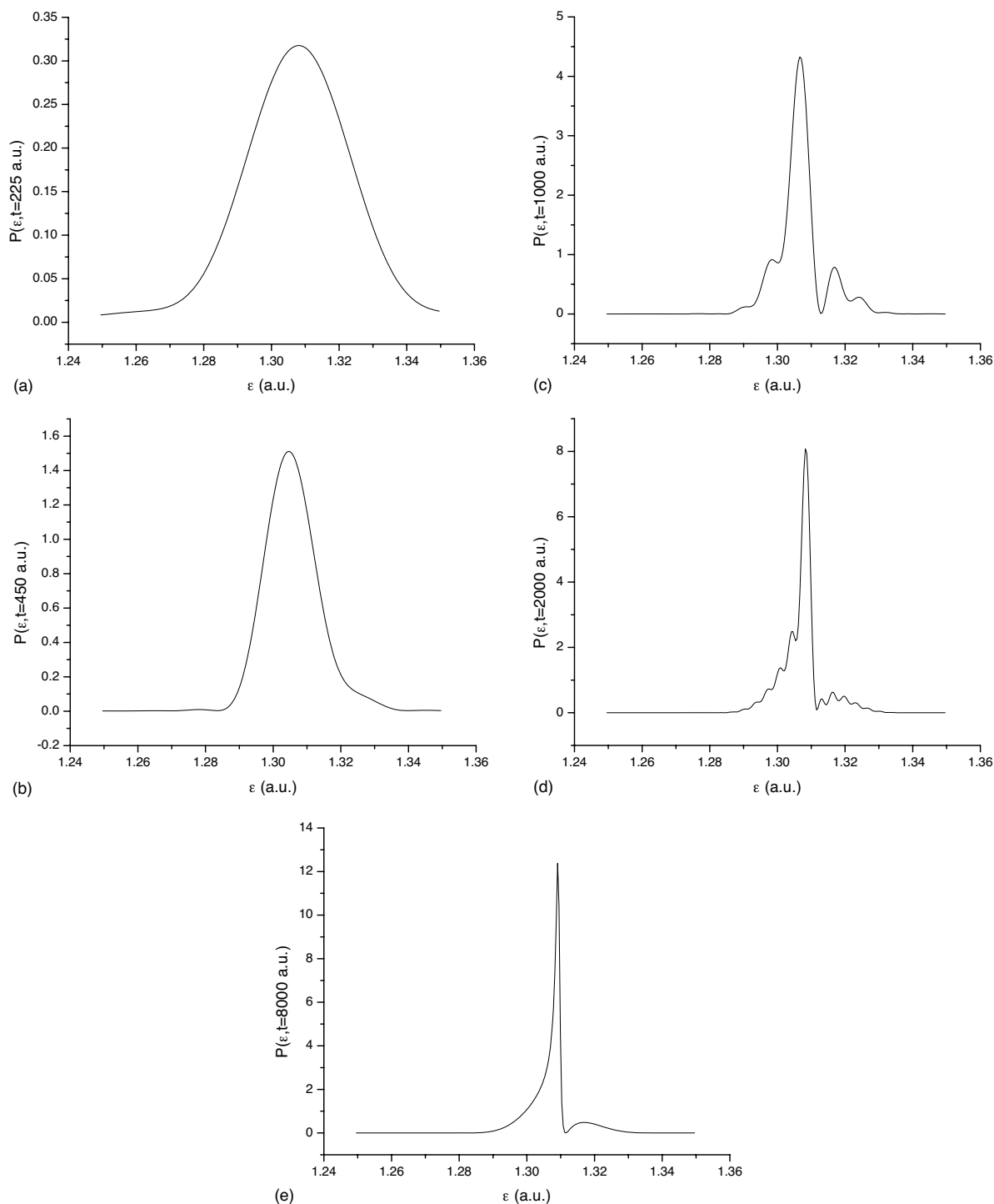
FIG. 3. (a) Time-resolved formation of the asymmetric profile of the differential ionization probability of the He 2s2p\ ^1P^o resonance state for excitation from the ground state with a pulse whose characteristics are given in the caption of Fig. 1 and in the text. For t=225 a.u. (b) As in (a), for t=450 a.u. (c) As in (a), for t=1000 a.u. (d) As in (a), for t=2000 a.u. (e) As in (a), for t=8000 a.u.
