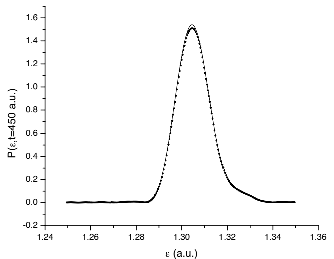
FIG. 2. Comparison between the SSEA and the analytic results, for field strength F=0.4 \times 10^{-1} a.u. at the end of the duration of the pulse ( t=450 a.u.). There is a minute discrepancy at the maximum, suggesting the beginning of the deviation of the FOTDPT [Eq. (32)] (solid line), from the nonperturbative approach.
