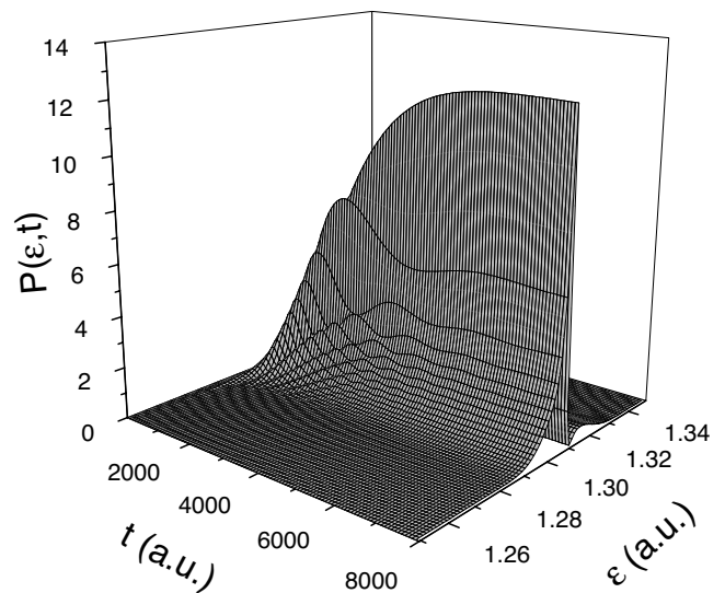
FIG. 1. The differential ionization probability, P(\varepsilon, t) , computed by the SSEA in this work, for the excitation of the He 2s2p^{-1}P^o resonance state. \varepsilon is the energy above the ionization threshold. The scattering wave function represents a nonstationary state, whose projection on the solution of the TDSE reveals the time-resolved excitation profile, with its characteristic asymmetric profile [see Eq. (32)]. The laser pulse has a \sin^2 envelope and duration of 450 a.u. ( \approx 11 fs). At the frequency of the excitation energy it contains 158 cycles. This profile is the same for field strengths in the range F=0.4 \times 10^{-3} a.u. to F=0.4 \times 10^{-1} a.u., apart from the modulating factor G(E, t) , given by Eqs. (23) and (34), which depends linearly on field strength F .
