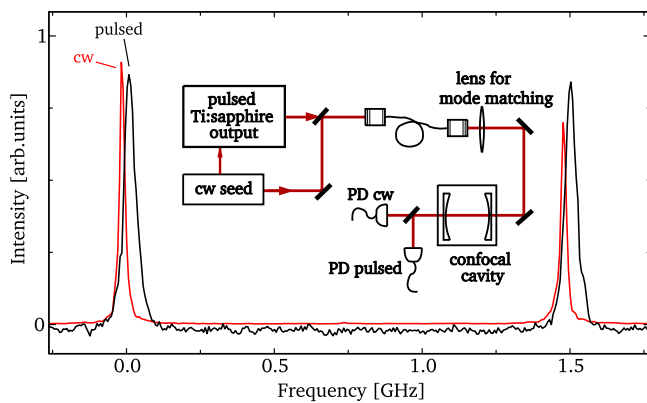
FIG. 7. (Color online) Measurement of the net frequency shift between the output of the CW seed laser and that of the pulsed oscillator (for one specific setting of the Hänsch-Couillaud lock on the cavity). As the seed light is tuned the etalon fringes (FSR = 750 MHz) of the pulsed output are redshifted from the CW fringes by 20 MHz. The experimental setup is given as an inset. Both the pulsed and the CW light are superimposed and mode matched by transmitting them through a single-mode fiber.
