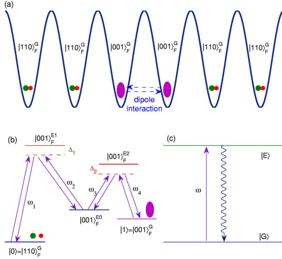
FIG. 1. (Color online) Scheme of quantum computation using diatomic qubits with conditional dipole-dipole interaction. (a) Diatomic qubits in one-dimensional optical lattices. The dipole-dipole interaction appears when neighboring bits occupy molecular states. (b) Single-bit operation with optimally controlled processes sandwiched Raman transition (see text). (c) Read-out with photon scattering (see text).
