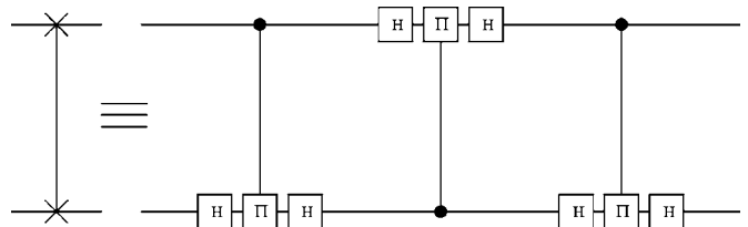
FIG. 1. Decomposition of the SWAP gate from C-phase( \pi ) gates and Hadamard (H) gates on the two qubits.
