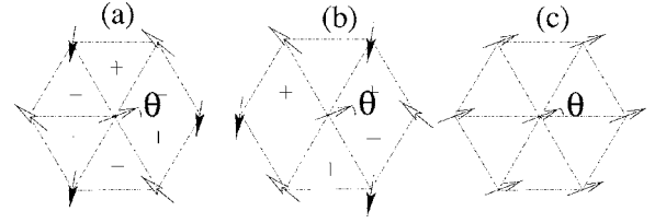
FIG. 7. (a) Classical ground-state configuration for J < 0 (configuration A). (b), (c) Classical ground-state configurations for J > 0 (configuration B and ferromagnetic configuration). The +, - signs denote the chirality of the triangular plaquettes (19).
