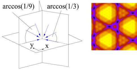
FIG. 1. (Color online) Scheme of the proposed experimental setup. Each arrow depicts a wave vector of a standing-wave laser. The three vertical planes intersect at an angle of 120^\circ . Dark (dark blue in the online version) spots in the right kagomé figure indicate the potential lattice minima.
