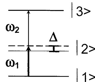
FIG. 1. A schematic of the atomic three-level system
