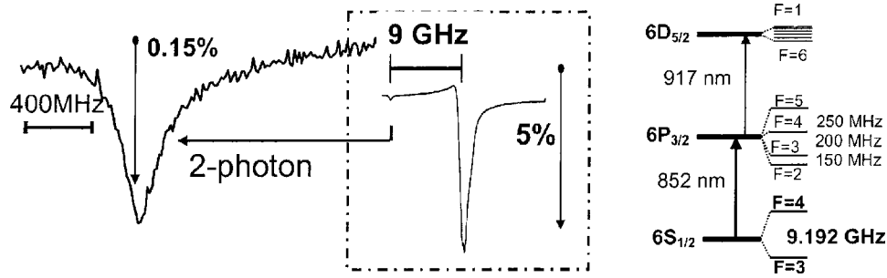
FIG. 4. Transmission spectrum recorded across the excited transition 6P_{3/2}-6D_{5/2} (917 nm) in a counterpropagating geometry on a 315-nm-thick Cs cell ( T=220^\circ\text{C} ) with the pump beam locked onto the 6S_{1/2}(F=3)-6P_{3/2} transition. The spectrum on the left is a zoom on the auxiliary resonance corresponding to the two-photon resonance 6S_{1/2}(F=4)-6D_{5/2} . The pump frequency is locked to the 6S_{1/2}(F=3)-6P_{3/2} transition. The hyperfine structure of the 6S_{1/2}-6P_{3/2}-6D_{5/2} levels is also shown.
