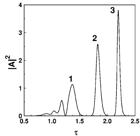
FIG. 10. ML pulse shape. (1) \alpha_g=1.0 ; (2) \alpha_g=2.0 ; (3) \alpha_g=3.0 . Other parameters are the same as in Fig. 9.
