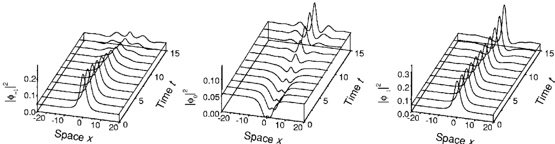
FIG. 7. The same as in Fig. 6, for the finite-background soliton (25). Parameters are \nu = a = 1 and \mu = -0.36 .
