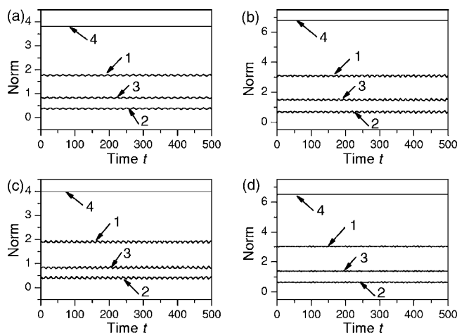
FIG. 5. The evolution of the three-component polar soliton (22) with initially added random perturbations. Parameters are \nu=1 , \mu_{+1}=-1.21 , and \mu_{-1}=-0.25 and (a), (c) a=0.5 and (b), (d) a=-0.5 . In cases (a) and (b), the random perturbation was added to the \phi_0 component and in cases (c) and (d) to components \phi_{\pm 1} . The curves marked by 1, 2, 3, and 4 depict, respectively, the evolution of the norms N_{+1} , N_{-1} , N_0 , and N ; see the definitions in Eqs. (15) and (4).
