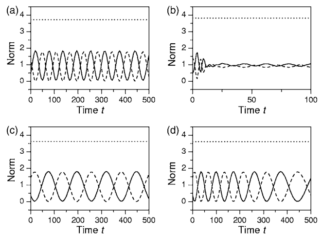
FIG. 4. The same as in Fig. 3 for the three-component polar soliton (21). Parameters are \nu=1 , \mu=-0.8 , and \epsilon=2/\sqrt{5} and (a) a=0.5 , (b) a=1.5 , (c) a=-0.5 , and (d) a=-1.5 . The meaning of the solid, dashed, and dotted curves is the same as in Figs. 2 and 3.
