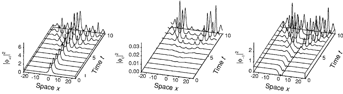
FIG. 6. The evolution of the two-component polar soliton on the cw background, Eq. (24), under the action of initial random perturbations added to the \phi_0 and \phi_{\pm 1} components. Parameters are \nu=+1 , a=-1/2 , and \mu=-1 .
