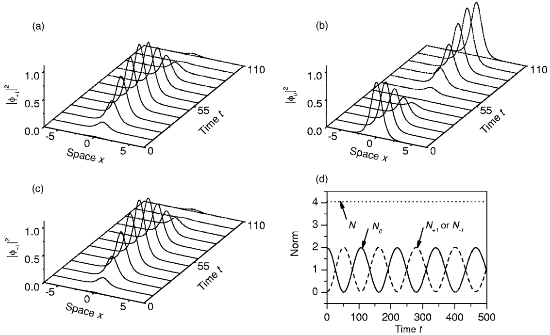
FIG. 1. Evolution of the single-component polar soliton (11) with a small random perturbation added, at t=0 , to the \phi_{+1} and \phi_{-1} components. Parameters are \nu=1 , a=-0.5 , and \mu=-1 .
