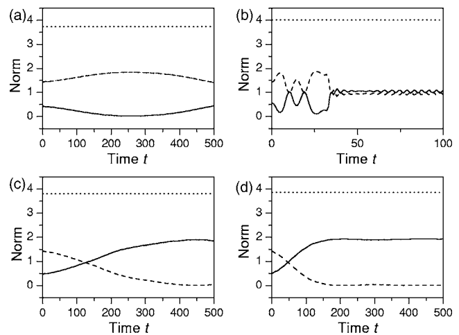
FIG. 3. The evolution of the three-component polar soliton (20) under the action of a small random perturbation initially added to the \phi_0 component. Parameters are \nu=1 , \mu=-0.8 , and \epsilon=2/\sqrt{5} and (a) a=0.5 , (b) a=1.5 , (c) a=-0.5 , and (d) a=-1.5 . The meaning of the solid, dashed, and dotted curves is the same as in Fig. 2.
