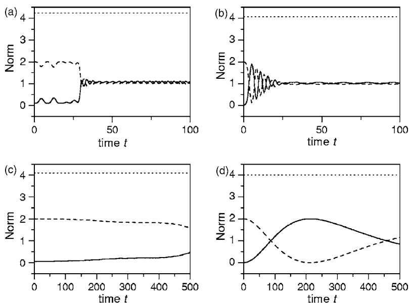
FIG. 2. The solid, dashed, and dotted curves show, respectively, the evolution of the norms N_0 , N_{\pm} of the \phi_0 and \phi_{\pm 1} components, and total norm N [see Eqs. (15) and (4)] in the two-component polar soliton (16) perturbed by a small random perturbation introduced in the \phi_0 component. Parameters are \nu=1 and \mu=-1 and (a) a=1.5 for \phi_{+1}\phi_{-1}^* < 0 , (b) a=1.5 for \phi_{+1}\phi_{-1}^* > 0 , (c) a=-1.5 for \phi_{+1}\phi_{-1}^* < 0 , and (d) a=-1.5 for \phi_{+1}\phi_{-1}^* > 0 .
