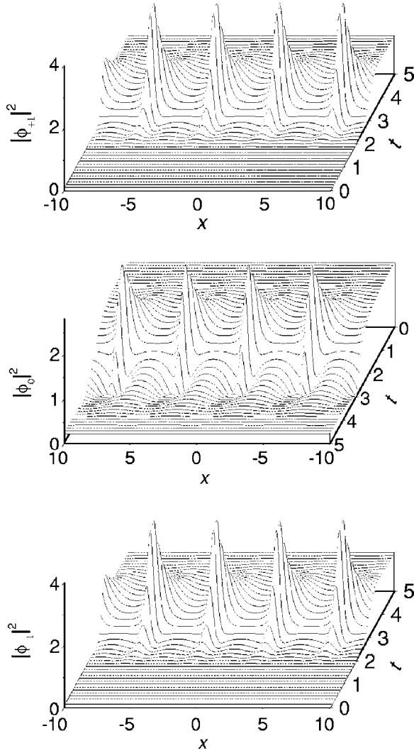
FIG. 8. The nonlinear development of the modulation instability, as per the exact solution (35), under the conditions k=2\eta and \alpha_c^2 + \beta_c^2 > \xi^2 . Parameters are k=0.6 , \eta=0.3 , \xi=1 , \alpha=\beta=\gamma=e^{-8} , \alpha_c=1.2 , and \beta_c=0 .
