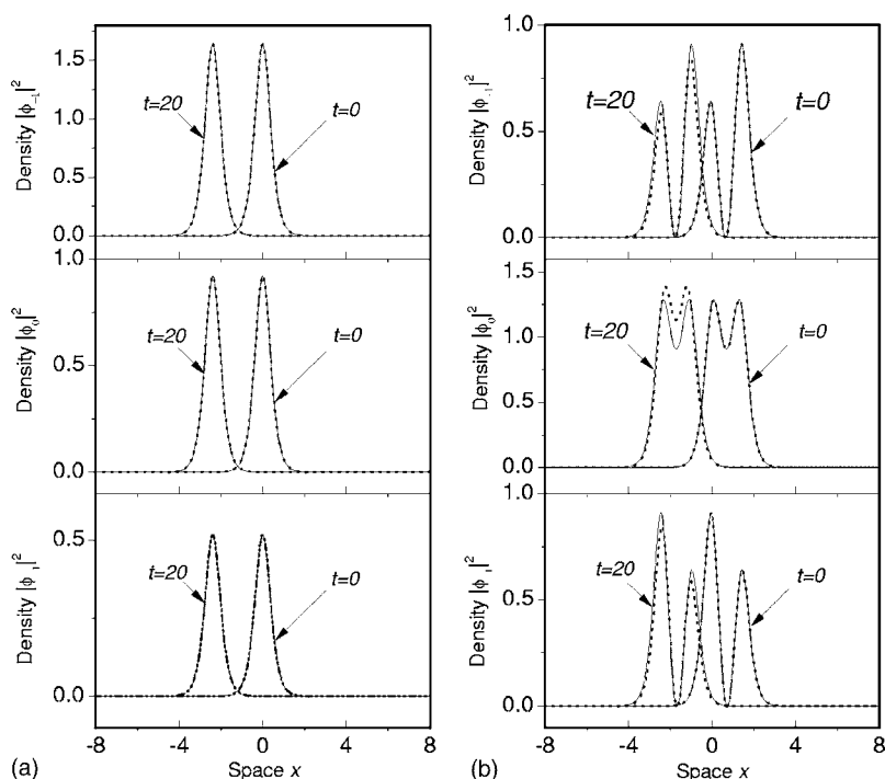
FIG. 9. The evolution of the density distribution in the soliton obtained from solution (35) by adding a randomly time-dependent perturbation of the nonlinear-coupling constant a , with the perturbation amplitude \pm 5\% . Parameters are \nu = a = 1 (as concerns the unperturbed value of a ), \xi = 1 , \eta = -0.03 , and \theta_0 = 0 . (a) The FM soliton, with \alpha_1 = 0.48 , \beta_1 and \gamma_1 being determined by conditions \alpha_1^2 = \beta_1 \gamma_1 and 2|\alpha_1|^2 + |\beta_1|^2 + |\gamma_1|^2 = 1 ; (b) the polar soliton, with \alpha_1 = 0.53 and \beta_1 = 0.43 , \gamma_1 being determined by 2|\alpha_1|^2 + |\beta_1|^2 + |\gamma_1|^2 = 1 . The solid and dotted curves show, respectively, the exact solutions and the perturbed ones produced by numerical simulations.
