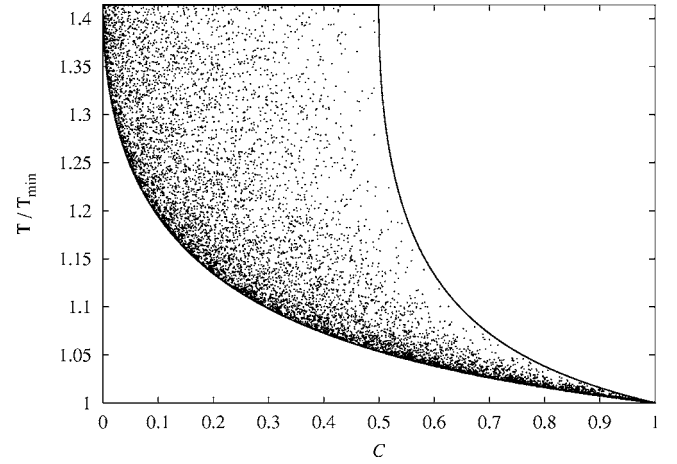
FIG. 1. Curves in the (C, \tau/T_{min}) plane corresponding, for each value of C , to the states of two (distinguishable) qubits with maximum and minimum \tau/T_{min} . The points represent randomly generated individual states that evolve to an orthogonal state. All depicted quantities are dimensionless.
