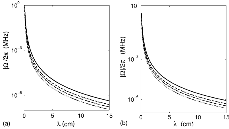
FIG. 1. Rabi frequency |\Omega| versus the microwave wavelength \lambda for a full-wavelength cavity (a) and a quarter-wavelength cavity (b) with ratios E_{\text{ch}}/E_J=4 (top solid line), 7 (dashed line), 10 (dash-dotted line), and 15 (bottom dotted line), respectively.
