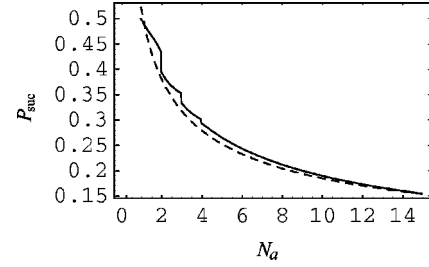
FIG. 2. The success probability of getting N_a photodetection events as a function of the number of atoms (solid line), fitted by the functional form C/N_a^{0.45} (dashed line) for some constant C . Unit detection efficiency is assumed.
