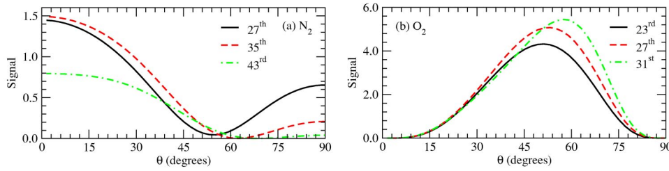
FIG. 1. (Color online) Predicted angular dependence of selective high-order harmonic yields in the plateau region for (a) N_2 and (b) O_2 . The angle is between the molecular axis and the laser polarization direction. For the laser parameters used, see text.
