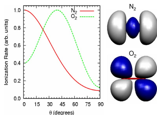
FIG. 2. (Color online) Angular dependence of the ionization rates for N_2 and O_2 calculated from the MO-ADK theory, and plots of the \sigma_g orbital of N_2 and the \pi_g orbital of O_2 .
