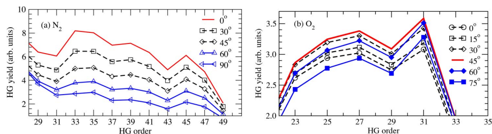
FIG. 3. (Color online) High-order harmonic yields at different angles predicted for the typical pump-probe experiments for N_2 and O_2 molecules. The angle is between the polarizations of the pump and probe lasers. The laser parameters are given in the text.
