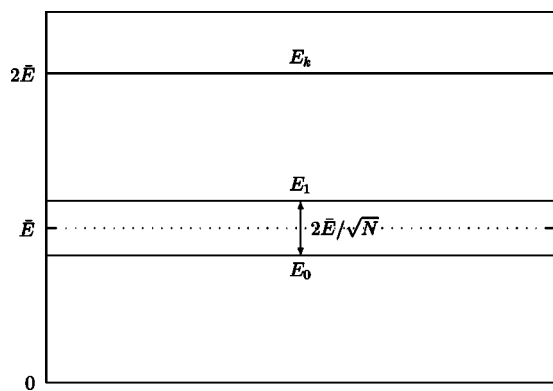
FIG. 1. Spectrum of the unperturbed Hamiltonian \bar{H}=H_0+H_f .
