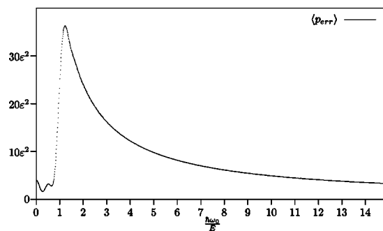
FIG. 2. Average error probability \langle p_{\text{err}} \rangle (to the second order) due to a noise modeled as in Sec. II with an autocorrelation function f(x)=\sin x/x for the analog search among N=100 elements. Note that \langle p_{\text{err}} \rangle stays very small as long as \hbar\omega_0/\bar{E} < 1 , at which point it shows a sudden increase. For larger values of \hbar\omega_0 , it tends progressively back to a low value. The peak at \hbar\omega_0 \sim \bar{E} scales as \sqrt{N} .
