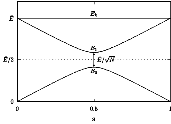
FIG. 3. Instantaneous eigenvalues of \tilde{H}(s) for N=32 .
