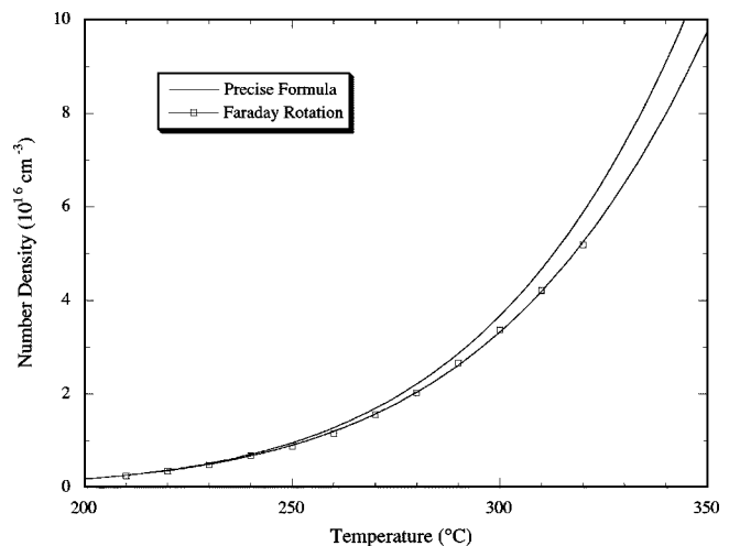
FIG. 5. Comparison of Cs number density calculated using the “precise” formula from Ref. [23] with that obtained from the Faraday rotation data. A curve of the same functional form has been fit to the Faraday data.
