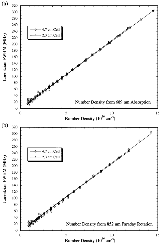
FIG. 6. Results for the collisional broadening, plotted vs the number density derived from (a) absorption on the 689 nm transition, and (b) Faraday rotation on the 852 nm transition. Straight line fits are shown through the data points, and the error bars on each point are smaller than the markers.
