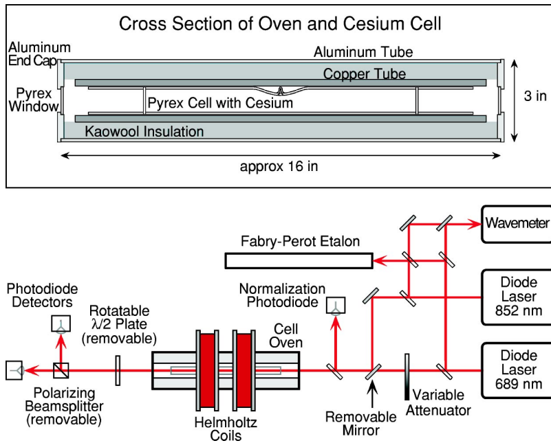
FIG. 2. (Color online) Diagram of the experimental apparatus, with an inset showing details of the oven and cesium cell.
