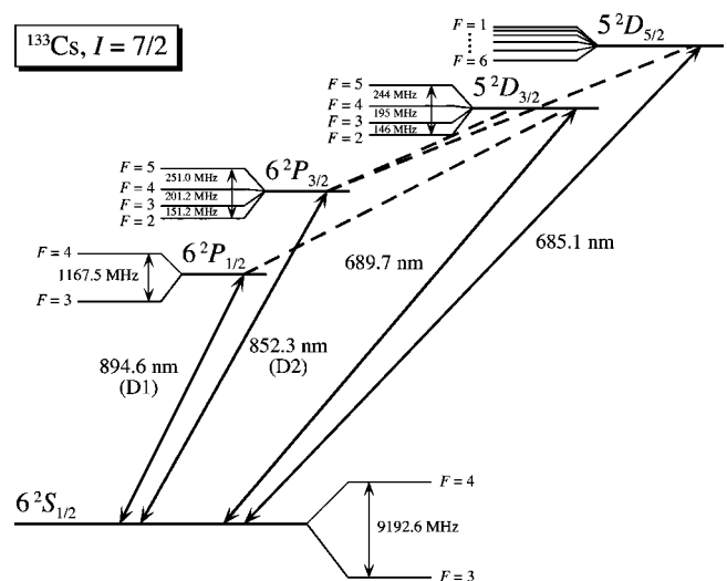
FIG. 1. The lowest energy levels and transitions in cesium, including the 689 nm and 852 nm lines of primary interest in this work. Dashed lines show the electric-dipole allowed transitions out of the 5D states. Hyperfine splittings are also shown for each state.
