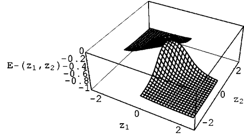
FIG. 6. E_-(z_1, z_2) for a constant magnetic field on the right side, plotted for particles on opposite sides of the origin.
