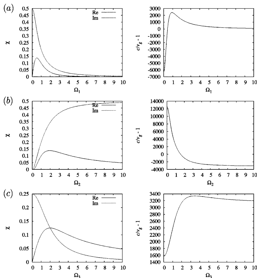
FIG. 4. Intensity tuning of group velocity: The general parameters are \Omega_1=\Omega_2=\Omega_3=\gamma , \gamma_1=\gamma_2=2\gamma . (a) Variation vs \Omega_1 , (b) variation vs \Omega_2 , (c) variation vs \Omega_3 . We note that only \Omega_2 provides maximum control over the group velocity of the probe pulse, as it allows switching the group velocity from subluminal to superluminal very much like the observation of Agarwal et al.
