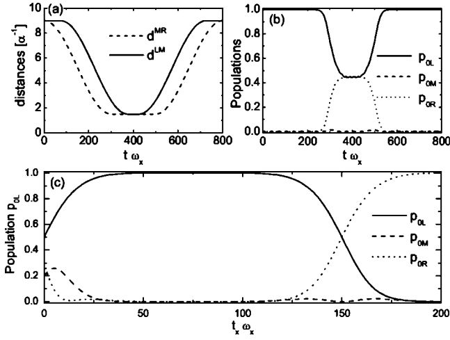
FIG. 4. (a) Approaching sequence for an EIT-like process, and (b) corresponding ground-state populations; d_{\text{max}}^{\text{LM}}\alpha = d_{\text{max}}^{\text{MR}}\alpha = 9 , d_{\text{min}}^{\text{LM}}\alpha = d_{\text{min}}^{\text{MR}}\alpha = 1.5 , t_r^{\text{LM}}\omega_x = t_r^{\text{MR}}\omega_x = 300 , t_i^{\text{LM}}\omega_x = 50 , t_i^{\text{MR}}\omega_x = 200 , and t_{\text{delay}}\omega_x = 120 . (c) Ground-state populations as a function of the time delay.
