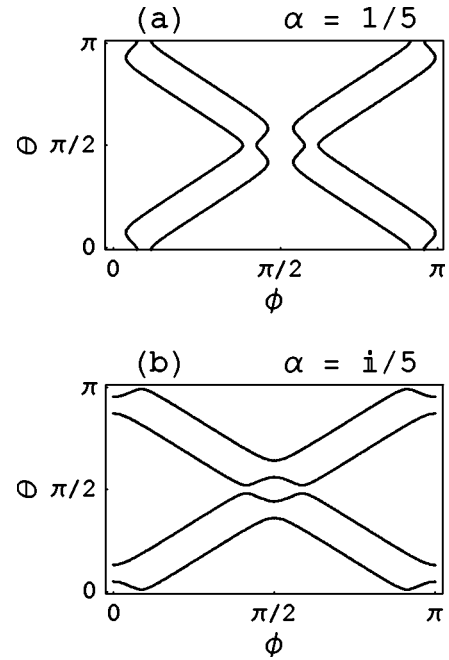
FIG. 12. Illustrating the effect of nonunitarity on the frequency band structure. Two band structures are shown, calculated for an OPO with G = \sqrt{2} , R = 0.5 and (a) t = \exp(-1/5) and (b) t = \exp(-i/5) . The two band structures have the same shape but they differ by a \pi/2 rotation in the plane of the figure.
