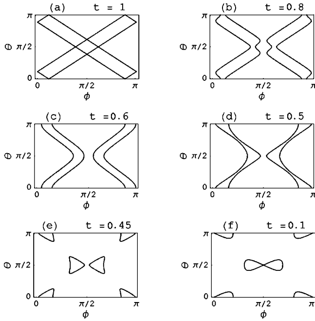
FIG. 11. Frequency band structures of an OPO in a cavity with nonorthogonal eigenmodes. The cavity “length” \theta = \omega L/c is plotted versus the rotator angle \phi for several values of the absorber parameter t . The values of the other parameters are G = \sqrt{2} , R = 0.5 .
