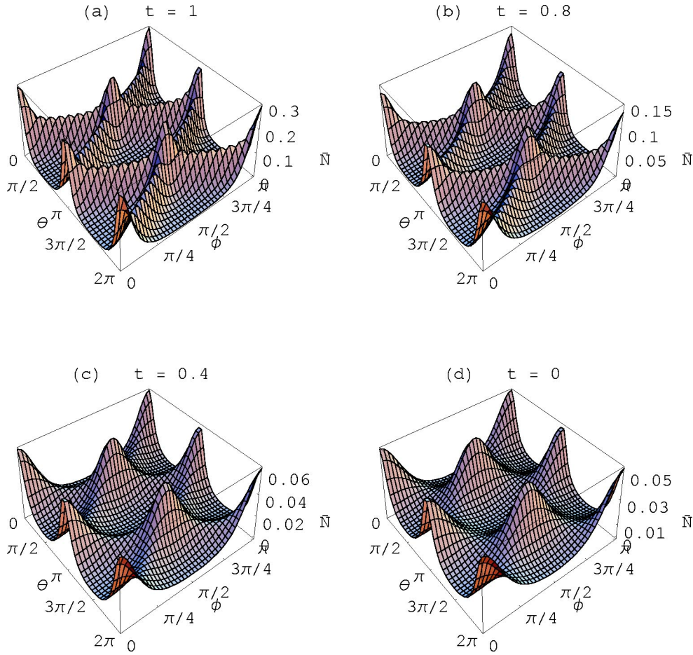
FIG. 6. Emission spectrum \bar{N}(\theta, \phi) for a subthreshold OPO calculated for G=1.01 , R=0.2 , and different values of t . (a) For a cavity with orthogonal modes ( t=1 ) we have the periodic behavior characteristic of the spectrum of a Fabry-Pérot cavity, but only so for \phi=0 and \phi=\pi/2 . For other values of \phi two resonant peaks for free spectral range appear. (b) and (c) For a cavity with nonorthogonal modes ( t < 1 ), \bar{N}(\theta, \phi) decreases with respect to the t=1 case but the doubling of the resonant peak remains.
