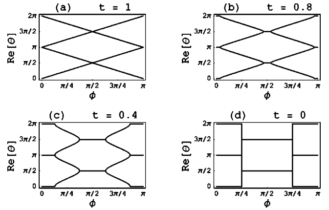
FIG. 8. Frequency band structures corresponding to the three-dimensional spectra shown in Fig. 6. We have plotted \text{Re}(\theta_{res}) versus the rotator angle \phi for different values of t .
