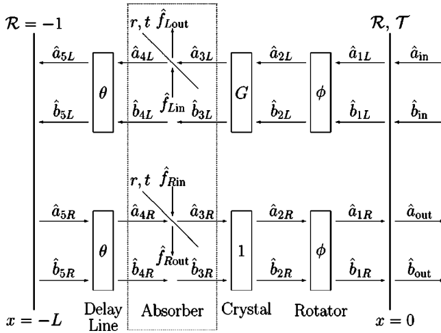
FIG. 1. Schematic representation of the degenerate-cavity parametric amplifier. Modes a and b have orthogonal polarizations. The boxes indicated with \phi , G , and \theta represent the rotator, the nonlinear crystal, and the delay line, respectively. In the dotted box we show the absorber modeled as a beam splitter acting only on mode a . For right-traveling modes we have put G=1 to indicate the passive crystal behavior when there is no phase matching.
