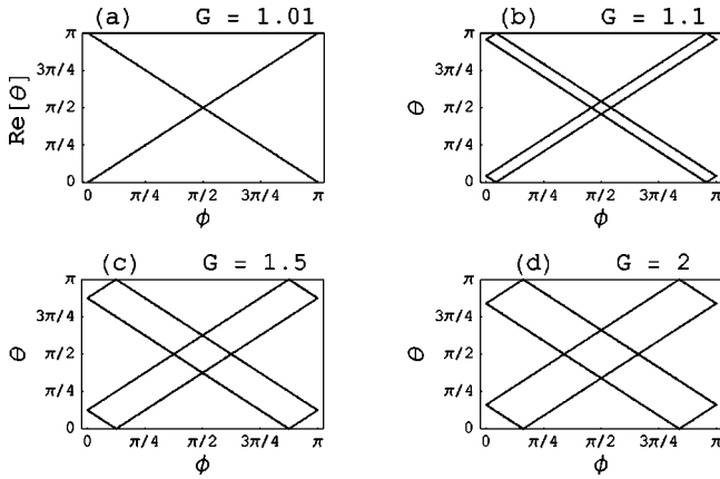
FIG. 9. Illustrating the doubling mechanism for an OPO in a cavity with orthogonal eigenmodes ( t=1 ) and mirror reflectivity R=0.5 . For increasing values of G the gap between bands is also increasing. Higher values of G are not considered here because our model is limited by the nondepleted pump approximation.
