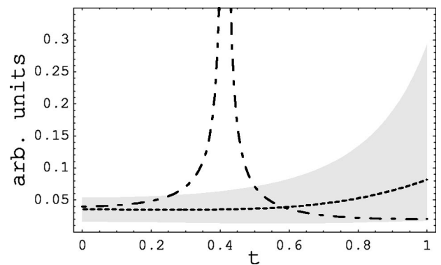
FIG. 5. Dotted-dashed line: “geometrical” Petermann K factor, given by Eqs. (47) and (48) for a cavity without crystal, calculated for \phi = \pi/8 , as a function of the absorber transmission t . The value of K diverges for t \rightarrow t_c(\phi = \pi/8) \approx 0.41 . Dashed line: total average photon number \bar{N} calculated at resonance and \phi = \pi/8 . The values of the other parameters are G=1.01 , R=0.2 , corresponding to a subthreshold OPO. The gray band represents all possible values of \bar{N} for nonorthogonal modes. Note that \bar{N} is not enhanced for t=t_c .
