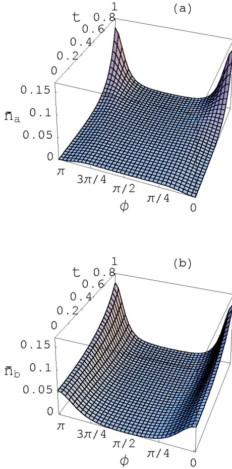
FIG. 3. (a) Plot of the average number \bar{n}_a of photons emitted on mode a for a subthreshold OPO at resonance as a function of the rotator angle \phi and the absorber parameter t . The values of the other parameters are G=1.01 , R=0.2 . For t=0 and \phi=0 the photons in mode a are fully absorbed so that \bar{n}_a=0 . (b) Plot of the average number \bar{n}_b of photons emitted in mode b under the same conditions as in (a).
