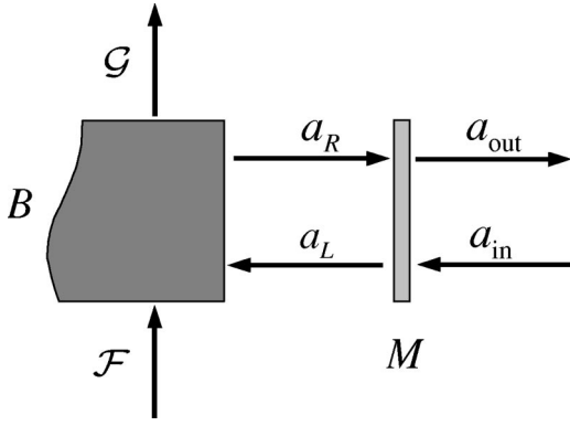
FIG. 7. Generalized one-output-mirror cavity. A mirror M is put in front of a bulk material B . The sets of annihilation field operators inside and outside the cavity are written as a_R, a_L and a_{out}, a_{in} , respectively. Analogously \mathcal{F}(\mathcal{G}) represents the set of annihilation input (output) noise operators.
