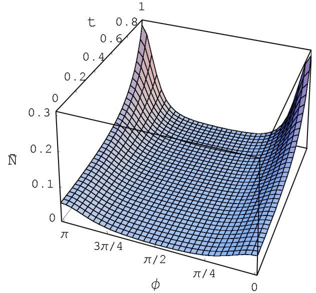
FIG. 4. Plot of the total average photon number \bar{N} \equiv \bar{n}_a + \bar{n}_b of the subthreshold OPO, calculated at resonance, as a function of the absorber transmission t and of the rotator angle \phi . The values of the other parameters are: G=1.01 , R=0.2 . For t=0 and \phi=0 the photons in mode a are fully absorbed and the residual value of \bar{N} is due to contribution of only mode b .
