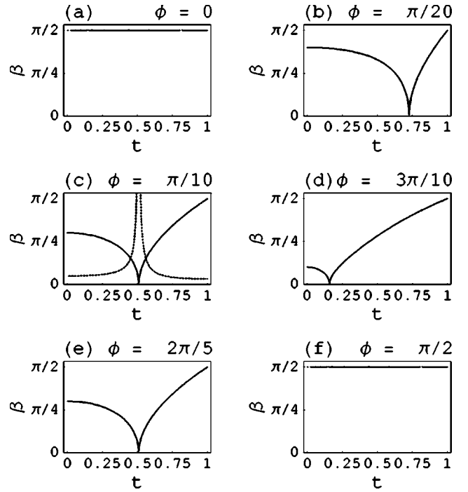
FIG. 2. (a)–(f) Angle \beta between the cavity eigenmodes \mathbf{u}_{\pm} versus the absorber parameter t for different values of the rotator angle \phi . For t=1 the eigenmodes are always parallel ( \beta=\pi/2 ) irrespective of the value of \phi . For t=t_c(\phi) the eigenmodes become parallel: \beta=0 . In (c) the dotted line gives the Petermann K factor ( \times 1/50 ) as calculated from Eqs. (47)–(48); the divergence appears for t=t_c(\phi=\pi/10)\approx 0.51 when the cavity eigenmodes are parallel.
