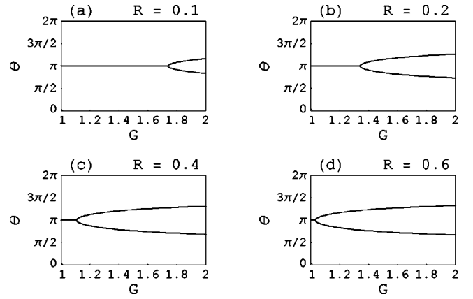
FIG. 10. Illustrating the bifurcation appearing around a single resonant peak in the OPO spectrum in a Fabry-Pérot cavity with orthogonal eigenmodes ( \phi=0 and t=1 ). When increasing the mirror reflectivity R the system approaches the threshold of oscillation for smaller values of G .
