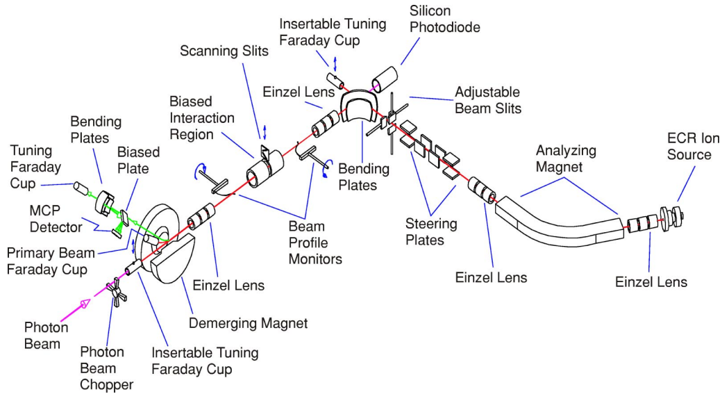
FIG. 1. Schematic of the ion-photon beam (IPB) end station at beamline 10.0.1 of the advanced light source (ALS).
