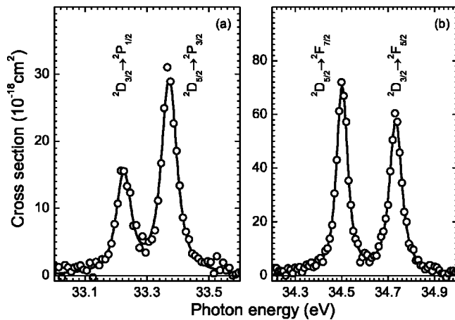
FIG. 5. Fits to the measured resonances due to 3p^6 3d^2 D \rightarrow 3p^5 3d(^3P)4s^2 P excitations (a) and 3p^6 3d^2 D \rightarrow 3p^5 3d(^3F)4s^2 F excitations (b) using the Voigt line profiles. The experimental energy spreads obtained from the fits are \Delta E = 22 \pm 3 meV (a) and \Delta E = 22 \pm 2 meV (b). Further results of the fits (full lines) are contained in Table II.
