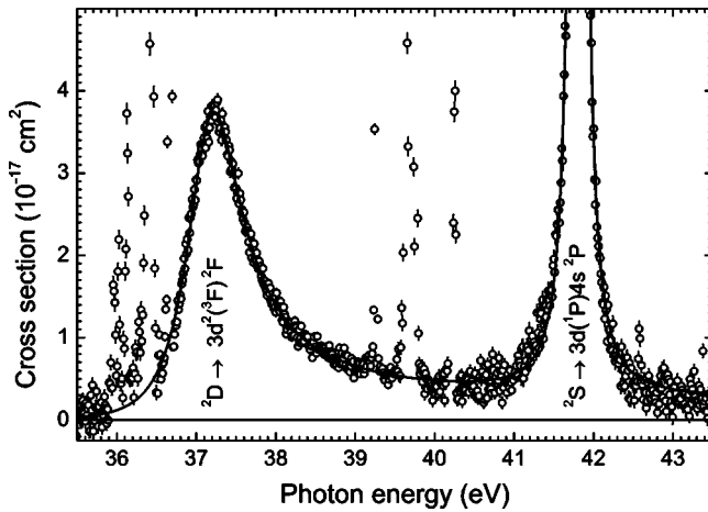
FIG. 8. The convolted Fano profile and the Voigt fit (full line) to the broad 3p^5 3d^2(^3F) ^2F and 3p^5 3d(^1P)4s ^2P resonances at 37.137 and 41.8065 eV, respectively. Due to the large natural widths of these resonances of 0.847 and 0.148 meV, respectively, their fine-structure splitting cannot be resolved. The 3p^5 3d^2(^3F) ^2F resonance exhibits a pronounced asymmetry. Its asymmetry parameter as obtained from the fit is 5.02 \pm 0.08 (see also Table II). The energy range of the fit was 35.5–43.5 eV. Narrow resonances in this range were individually excluded from the fit. The fitted experimental energy spread is \Delta E = 44 \pm 4 meV.
