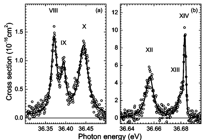
FIG. 7. The Voigt line profile fits (full lines) to high-resolution measurements (open symbols) in the photon energy ranges 36.3–36.5 eV (a) and 36.635–36.695 eV (b). From the fit (a) the experimental energy spread \Delta E = 1.87 \pm 0.08 meV is obtained. The same value has been used and kept fixed in fit (b). Further fit results are summarized in Table II, where the resonances are labeled by Roman numerals.
