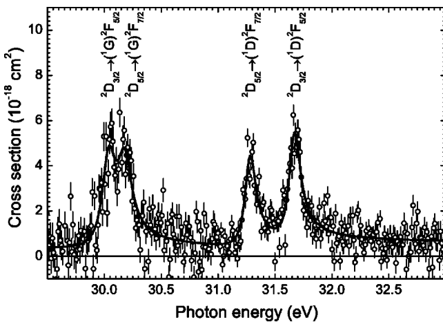
FIG. 4. Expanded view of the lowest-energy group of measured resonances associated with 3p^6 3d^2 D \rightarrow 3p^5 3d^2 {}^2F excitations. The resonances exhibit asymmetric line shapes which can be fitted by the Fano profiles convoluted with a Gaussian. The results of the fit (full line) are contained in Table II. In the fit, the experimental energy spread was kept fixed at \Delta E = 19 meV.
