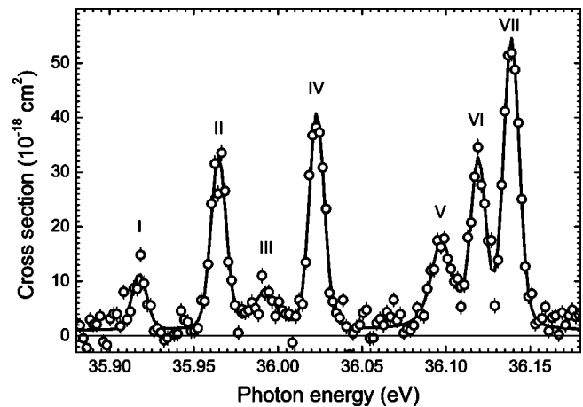
FIG. 6. The Voigt line profile fits (full lines) to measured PI resonances (open symbols) in the photon energy range 35.88–36.18 eV. The fitted experimental energy spread is \Delta E = 9.7 \pm 0.5 meV. Further fit results are summarized in Table II, where the resonances can be identified with the aid of the Roman numerals shown.
