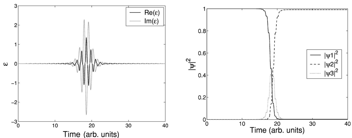
FIG. 4. Same as Fig. 3 but for \alpha=0.01 .
