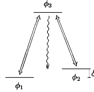
FIG. 1. Prototypical \Lambda -type level scheme used in our calculations: \phi_1 and \phi_2 are long-lived states, whereas \phi_3 is a short-lived state that is optically coupled to both \phi_1 and \phi_2 (for details see text); wiggled line indicates relaxation and dephasing of state \phi_3 .
