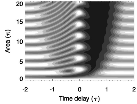
FIG. 2. Results of our calculations for the simplified model system described in the text, and using two laser pulses with Gaussian envelopes (with full width of half maximum \tau ). Before the pulse sequence the system is in state \phi_1 ; black (white) areas correspond to the situation that after the pulse sequence the population of \phi_2 is one (zero). Negative (positive) time delays correspond to the situation that the \epsilon_1 pulse excites the system before (after) the \epsilon_2 one, and the pulse area is defined as \int_{-\infty}^{\infty} dt g(t) (we use \mu_1 = \mu_2 = 1 and \gamma_o = 0.2\tau^{-1} ).
