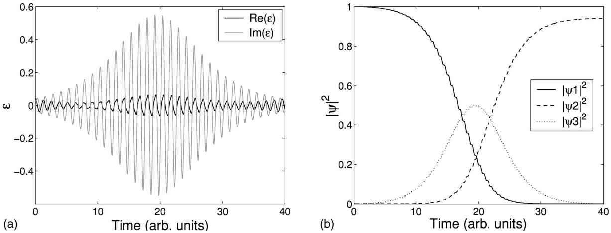
FIG. 3. Results of our optimal-control calculations for \gamma=0.001 , \alpha=0 ; (a) optimal control and (b) transients of \psi_1 , \psi_2 , \psi_3 .
