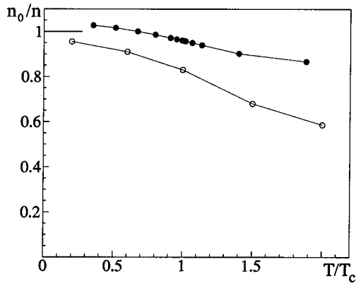
FIG. 8. Temperature dependence of n_0/n for mU=0.2 derived from universal relations (filled circles) and simulated for the quantum lattice BG (open circles). Points are connected with lines to guide the eye.
