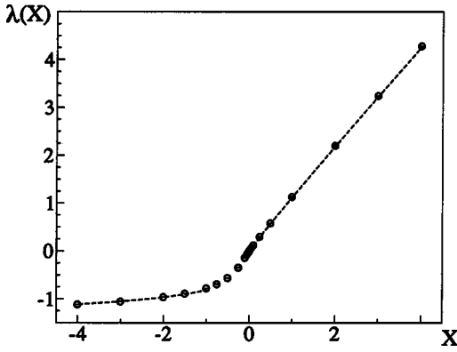
FIG. 2. The \lambda(X) function compared to its asymptotic large |X| expressions.
