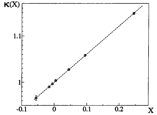
FIG. 4. RG parameter \kappa(X) obtained from finite-size scaling of the data according to Eqs. (34) and (35) and fitted using a linear in X expansion with d\kappa/dX = 0.61 .
