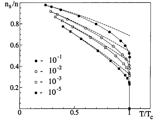
FIG. 6. Temperature dependence of n_s/n for small mU = 10^{-1}, 10^{-2}, 10^{-3}, 10^{-5} . Points are connected with lines to guide the eye. The dashed lines are the mean-field theory results with an exact relation between T_c and particle density.
