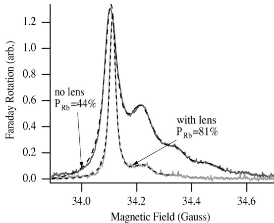
FIG. 2. Rb EPR spectra taken with divergent and collimated light. The main peak is the F=3, m=3 \rightarrow F=3, m=2 transition in ^{85}\text{Rb} , while the second peak is the unresolved F=3, m=2 \rightarrow F=3, m=1 and F=2, m=2 \rightarrow F=2, m=1 pair.
