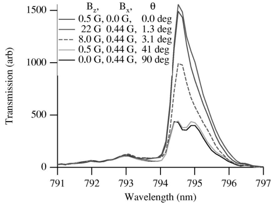
FIG. 1. Light transmission for various magnetic-field directions and magnitudes. The transverse field of 0.44 G is simply the Earth's field that is cancelled for the 0.5-G data.
