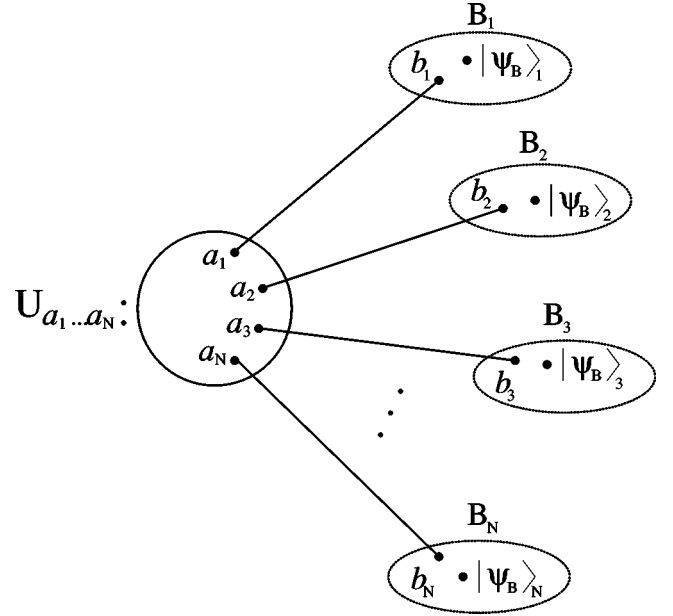
FIG. 3. Remote operation on N distributed systems.
