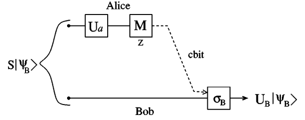
FIG. 2. Usage of a stator to operate a remote rotation.
