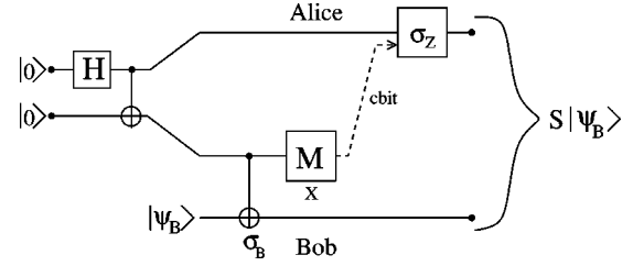
FIG. 1. Preparation of a stator acting on Bob's state.
