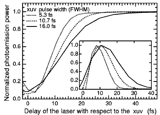
FIG. 6. Total power of photoemission from H at \hbar\omega>7.5\hbar\omega_L (normalized to unity at \Delta t=50 fs) vs delay \Delta t of the laser pulse ( \tau_L=10.7 fs, I_L=2\times 10^{13} W/cm ^2 ) with respect to the xuv pulse ( I_X=3\times 10^{10} W/cm ^2 ). Inset: the derivative of the total photoemission power with respect to \Delta t (normalized to unity at the peak of each curve).
