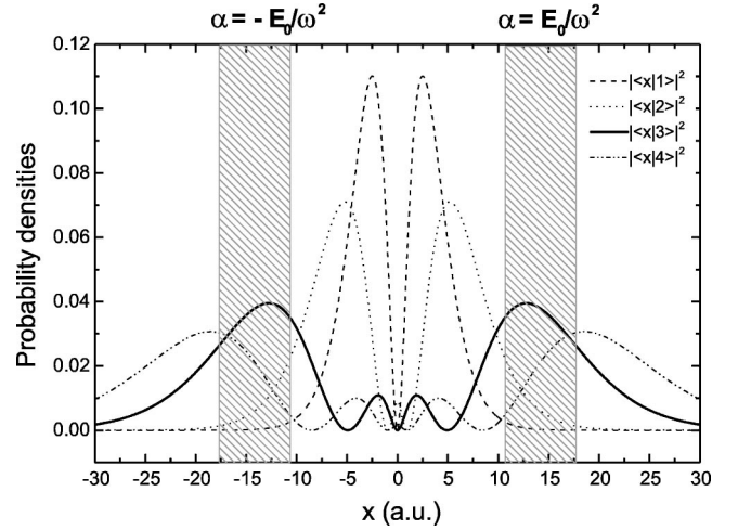
FIG. 3. The probability distributions |\langle x|n\rangle|^2 for the first four excited states of the untruncated potential (3). The range of excursion amplitudes \alpha = E_0/\omega^2 = 2\sqrt{\eta/\omega} that is covered in Fig. 2 (for 2.3 < \eta < 6.3 ) is shaded. Truncation has a minor effect for n=1 and 2. For n=3 , this effect is becoming noticeable, and for n=4 , it is strong. All higher excited states are eliminated by the truncations considered.
