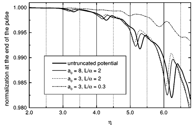
FIG. 4. Normalization of the time-dependent wave function at the end of the pulse as a function of \eta = U_p/\omega , for the truncation parameters of Table I. The pulse length is eight cycles plus a linear turn on of two cycles.
