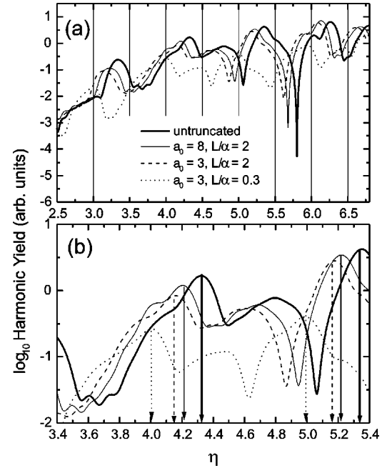
FIG. 2. Intensity of the 13th harmonic as a function of \eta = U_p/\omega . (a) Comparison between the untruncated and various truncated soft-core potentials; the two values of the parameter L , L = 31.78 a.u. and L = 4.77 a.u., correspond to 2\alpha(\eta = 4.8) and 0.3\alpha(\eta = 4.8) , respectively. The binding energies for the various truncated potentials are given in Table I. (b) Enlargement of part (a), for 3.4 < \eta < 5.4 . The values of this parameter, for which the enhancements are maximal, are marked by arrows.
