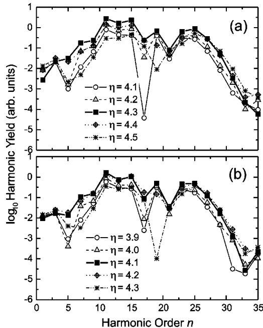
FIG. 1. Harmonic spectra for \omega = 0.076 a.u., \varepsilon_0 = 0.7566 a.u., and several values of \eta = U_p/\omega , for the untruncated (a) and truncated (b) soft-core potential, with L \approx 31.78 a.u. and a_0 = 3 a.u. The parameter L was chosen as twice as the electron excursion amplitude \alpha for \eta = 4.8 . The harmonic intensities are connected by lines to guide the eye. The thick lines correspond to the field intensity for which the enhancement is maximal.
