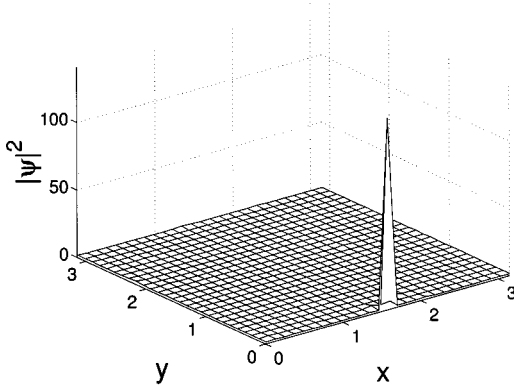
FIG. 2. Gaussian Klauder coherent state with a double Gaussian form factor. The parameter values are a=\pi , n_0=6500 , m_0=6500 , and \sigma=23 . A highly localized initial state can be seen.
