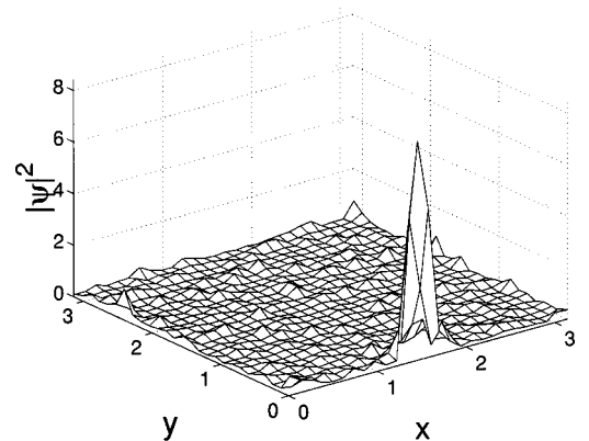
FIG. 5. This has the same initial wave packet as in Fig. 2. The wave packet has made five complete round-trips of the box in a counterclockwise direction.
