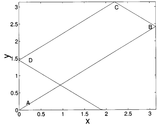
FIG. 7. A classical trajectory corresponding to the motion of the wave packet with parameters a=\pi , n_0=6500 , m_0=5000 , \sigma_n=23 , and \sigma_m=20 is shown. The impacts with the edges occur at corresponding positions. A plot of the corresponding positional expectation value for the quantum wave packet is indistinguishable.
