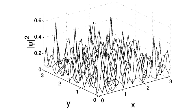
FIG. 1. Gaussian Klauder coherent state with a single Gaussian form factor. The parameter values are a = \pi , n_0 = 10\,000 , and \sigma = 5 . No localization is discernable.
