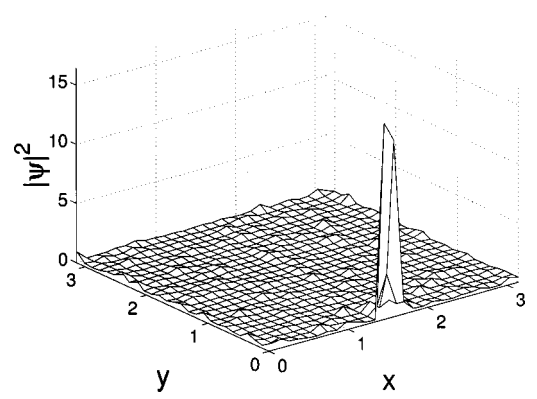
FIG. 4. This has the same initial wave packet as in Fig. 2. The wave packet has made three complete round trips of the box in a counterclockwise direction.
