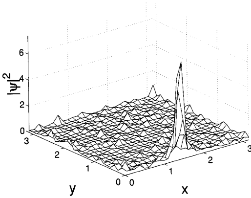
FIG. 6. This has the same initial wave packet as in Fig. 2. The wave packet has made seven complete round-trips of the box in a counterclockwise direction. Partial delocalization can be seen, and the peak height has decreased substantially.
