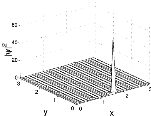
FIG. 3. This has the same initial wave packet as in Fig. 2. The wave packet has made one complete round-trip of the box, in a counterclockwise direction.
