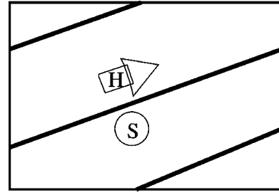
FIG. 3. S stays on Earth while H travels on the periodic orbit of Fig. 2.
