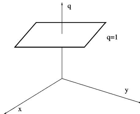
FIG. 1. The embedding of (3+1)-Minkowski space into (4+1)-Minkowski space. The (t,z) directions are suppressed so that the manifold appears as an infinite sheet fixed at q = 1 .
