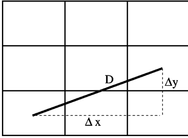
FIG. 2. The compact hypertorus can be represented as an identified parallelepiped. Alternatively, the compact topology can be represented by tiling flat space with identical copies of the fundamental parallelepiped. In the tiling picture above only the (x,y) directions are shown. A particular periodic orbit is drawn which corresponds to x_{\text{end}} = T_y T_x^2 x_{\text{start}} .
