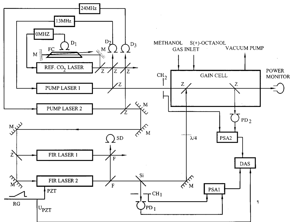
FIG. 1. The experimental setup. The ref. CO 2 laser is line-center stabilized using a CO 2 vapor fluorescence cell FC while D1 represents an InSb liquid-nitrogen-cooled detector. The pump laser 1 and pump laser 2 are off-center stabilized to pump the gain cell and the FIR lasers, respectively; D2 and D3 are HgCdTe liquid-nitrogen-cooled detectors. Frequency tuning of FIR laser 2 was accomplished by a PZT (piezo translator) driven by a ramp generator labeled RG. The beat frequency between the tunable FIR laser 2 and the center-frequency-fixed FIR laser 1 was monitored by a Schottky diode labeled SD. CH1 and CH2 are mechanical choppers, PSA1 and PSA2 are phase-sensitive amplifiers, and PD1 and PD2 are pyroelectric detectors. In all cases Z and F represent ZnSe and foil beam splitters while M represents metallic mirrors. All data were stored in the data-acquisition system DAS.
