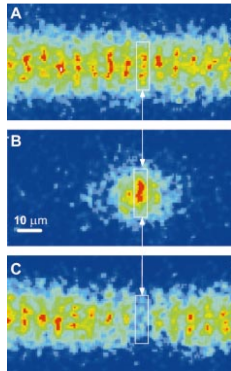
FIG. 3. (Color) Images of the lattice after the following manipulations: (A) no manipulation of the atoms in the microtraps; (B) only atoms from a single lattice site illuminated during the exposure with a focused laser beam; (C) after removing atoms in one lattice site before the exposure.
