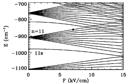
FIG. 1. Energy levels of m=0 states of Li as a function of static electric-field strength. These are energies around the n=11 manifold.
