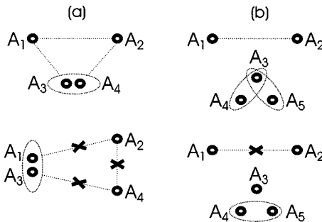
FIG. 3. (a) N=4 and \rho_{VI} is such that a GHZ state shared among the groups A_1-A_2-(A_3A_4) can be created if and only if the parties (A_3A_4) join, and no entanglement can be distilled if any other two parties form a group. (b) N=5 and \rho_{VII} is such that entanglement between A_1 and A_2 can be created if and only if either party (A_3A_4) or (A_3A_5) join, however no entanglement can be distilled if (A_4A_5) joins.
