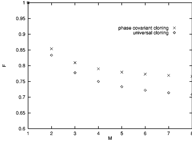
FIG. 1. Upper bound for the fidelity in phase-covariant cloning compared with the optimal fidelity for universal cloning of qubits. Both sets of points are shown for a fixed number of inputs, N=1 , as a function of M , the number of outputs. For the limit M \rightarrow \infty one finds from the formulas given in the text that \bar{F}_{pcc}(1, \infty) = 3/4 and F_{univ}^{opt}(1, \infty) = 2/3 .
