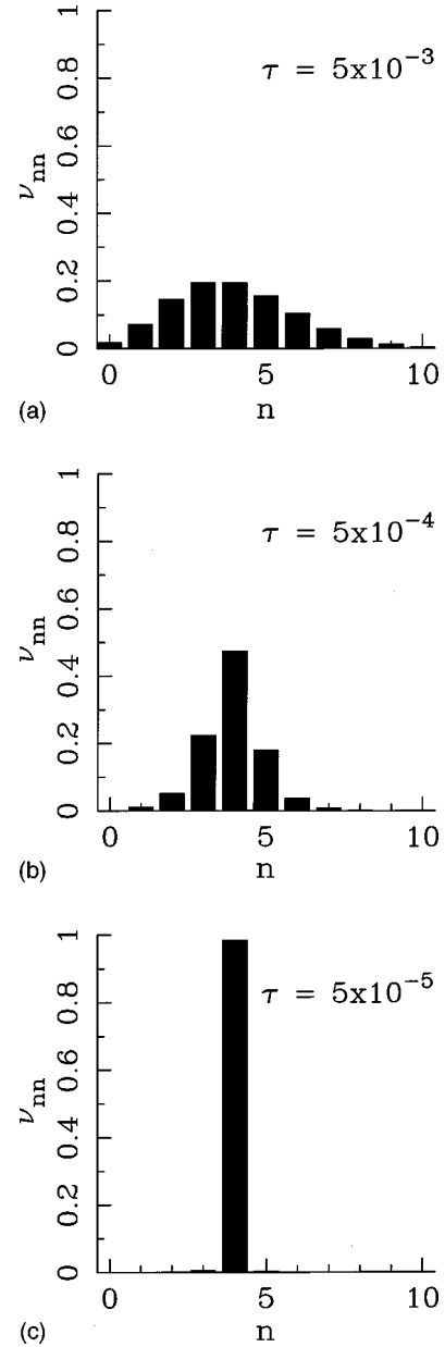
FIG. 2. The number distribution of the conditional output state \hat{\nu}_{out} for different values of the BS transmissivity \tau , indicated on each plot. The parameters are chosen to select the number state |n^* \equiv 4\rangle , with \chi t = 0.01 and \psi = 0.04 . The modes a_1 and c_1 are both excited in a coherent state with real amplitudes \alpha = 20 and \beta = 2 , respectively. The probabilities of obtaining the three states (i.e., the detection probability at D ) are respectively P_1 = 0.99885 , 0.4905 , 0.1997 .
