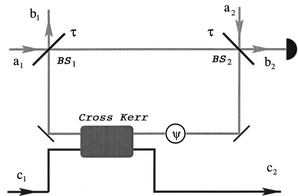
FIG. 1. Schematic diagram of the setup for the generation of Fock states and superposition of Fock states. BS_1 and BS_2 denote high-transmissivity beam splitters, and \psi a tunable phase shift. The cavity input modes a_1 and a_2 are in a coherent state and in the vacuum, respectively. The box denotes the cross-Kerr medium that couples the cavity mode d with the traveling free mode c_1 , which is initially prepared in a coherent state. After a successful detection at the photodiode D , which tests the presence of an output excited coherent field in mode b_2 , the output mode c_2 is found in a Fock state or in a superposition of a few Fock states.
