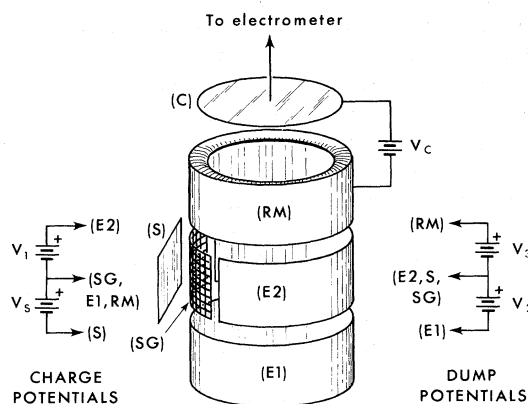
FIG. 3. Sketch of the cell used to study extraction of charge through the liquid meniscus. The liquid level is set near the top of the electrode RM.
