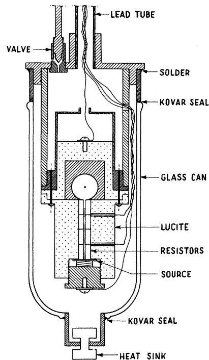
FIG. 5. Cross-section view of the assembled experimental cell.
