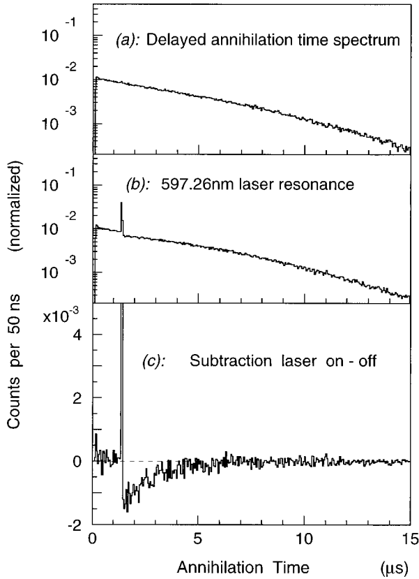
FIG. 4. (a) \bar{p} He + delayed annihilation time spectrum taken with 4 He gas target of 0.55 bar and 6.3 K. (b) 597.26-nm resonance induced at t = 1.35 \mu\text{s} on the time spectrum. (c) Depletion-recovery spectrum, the difference between the two normalized spectra (a) and (b).
