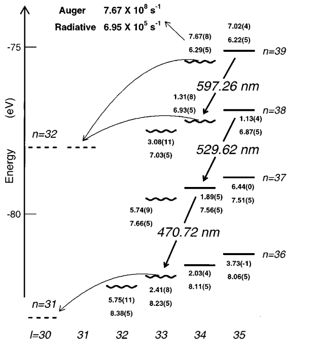
FIG. 2. Portion of the level structure of the \bar{p}^4\text{He}^+ atom, showing the positions of the experimentally observed 597.26-nm, 470.72-nm, and 529.62-nm resonances. The theoretical values for Auger [34] and radiative transition [27] rates of each state ( n, \ell ) are indicated.
