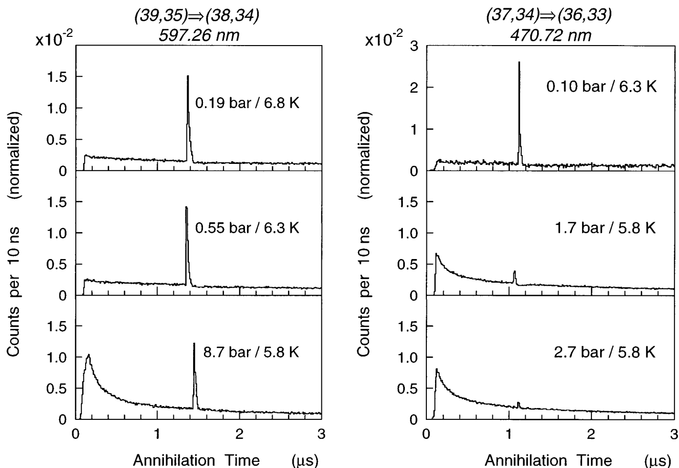
FIG. 7. Profiles of the two resonances (n,\ell)=(39,35)\rightarrow(38,34) at 597.26 nm (left), and (37,34)\rightarrow(36,33) at 470.72 nm (right), measured at various densities. The 597.26-nm resonance intensity is independent of density, whereas that of the 470.72-nm resonance diminishes as the density increases.
