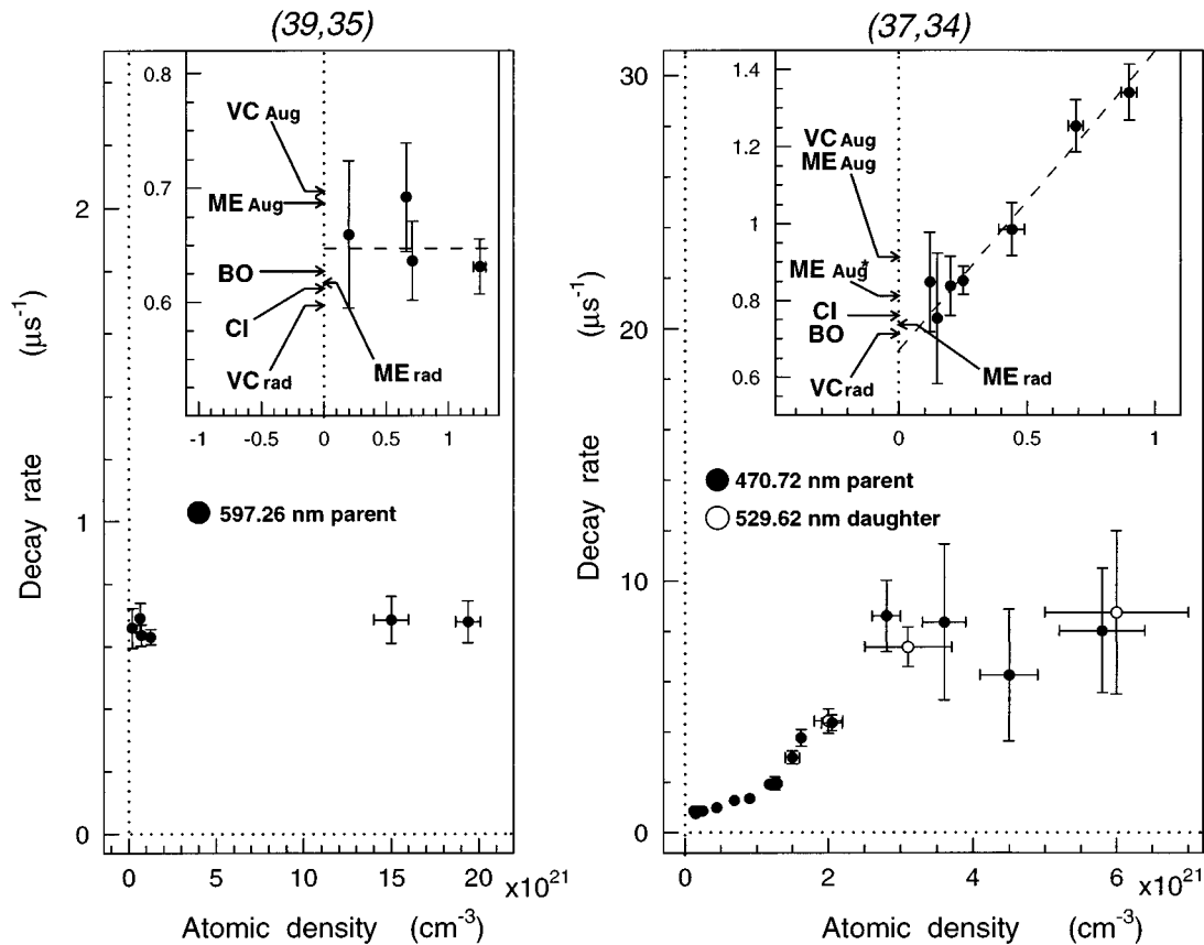
FIG. 12. Decay rates of the states (n,\ell)=(39,35) and (37,34) measured at various densities using the 597.26-nm, 470.72-nm, and 529.62-nm resonances. Radiative rates from Born-Oppenheimer (BO [26,27]) and variational calculations ( VC_{\text{rad}} [30] and ME_{\text{rad}} [33]) and the sum of Auger and radiative rates from atomic configuration-interaction (CI [24]) and variational calculations ( VC_{\text{Aug}} [30,31], ME_{\text{Aug}} [34], and ME_{\text{Aug}}^* [35]) are shown.
