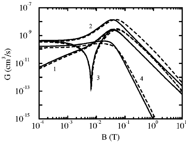
FIG. 5. Comparison of the CC calculation (solid lines) and the ABC approximation with R=40a_0 (dashed lines) for the exchange decay rate constants of the processes (1) 54 \rightarrow 63 , (2) 54 \rightarrow 52 , and (3) 54 \rightarrow 41 , (4) 54 \rightarrow 21 .
