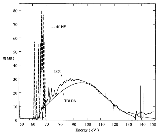
FIG. 8. Comparison between the experimental 4d \rightarrow nf, \varepsilon f spectrum of I^{2+} and the results of HF (discrete spectrum) and TDLDA calculations. The experimental spectrum was arbitrarily fitted to give best agreement with the TDLDA results.
