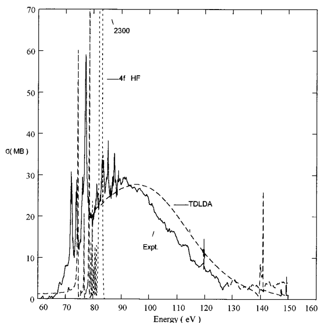
FIG. 9. Comparison between the experimental 4d \rightarrow nf, \varepsilon f spectrum of I^{2+} and the results of HF (discrete spectrum) and TDLDA calculations. The experimental spectrum was arbitrarily fitted to give best agreement with the TDLDA results. It should be noted that the experimental spectrum also contains some contributions from I^+ and I^{3+} .
