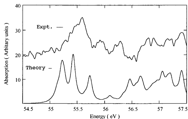
FIG. 5. Comparison between theory and experiment for the 4d \rightarrow 6p, 7p , etc., transitions in neutral iodine. Note the spectra agree best if the theoretical spectrum is shifted by \sim 0.15 eV towards higher energy.
