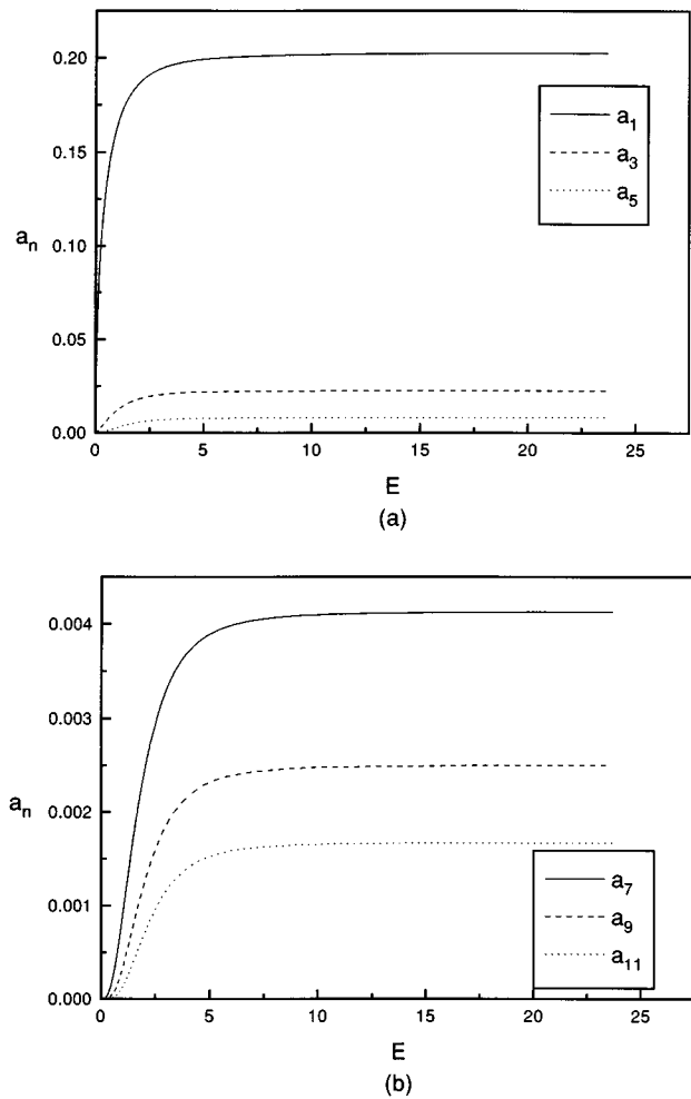
FIG. 4. (a) Fourier coefficients a_1, a_3 , and a_5 vs energy E . m = T = c = 1 . (b) Fourier coefficients a_7, a_9 , and a_{11} vs energy E . m = T = c = 1 .
