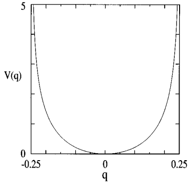
FIG. 1. Constant period potential. m=T=c=1 .
