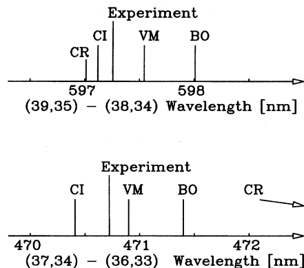
FIG. 2. Various theoretical predictions on the transition wavelength (BO, CI, VM, and CR; see the text for explanations) are compared with the experimental values for the two laser resonance transitions found in the previous and present experiments.
