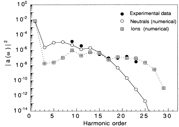
FIG. 6. Neutral [ \text{He} (dots)] and ion [ \text{He}^+ (squares)] response at I = 3.2 \times 10^{15} W/cm 2 . Experimental data (solid dots) from Ref. [5], normalized to the 13th harmonic, have been included for comparison.
