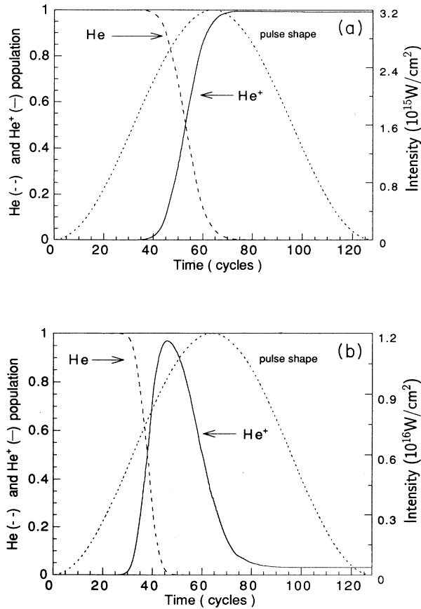
FIG. 5. (a) Neutral (He) and ion ( \text{He}^+ ) populations for a \sin^2 pulse profile of 128 cycles (105 fs) and peak intensity I = 3.2 \times 10^{15} W/cm 2 . (b) Neutral (He) and ion ( \text{He}^+ ) populations for a \sin^2 pulse profile of 128 cycles (105 fs) and peak intensity I = 1.2 \times 10^{16} W/cm 2 .
