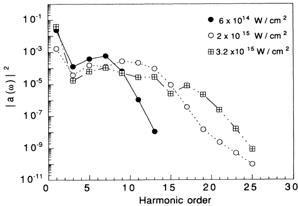
FIG. 3. Harmonic spectra of helium at intensities (a) I = 6 \times 10^{14} \text{ W/cm}^2 (solid dots), (b) I = 2 \times 10^{15} \text{ W/cm}^2 (dots), and (c) I = 3.2 \times 10^{15} \text{ W/cm}^2 (squares) for a short pulse with a linear turn on. For clarity we plot only the peak intensities of each harmonics joined by a line to guide the eye.
