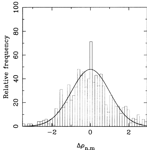
FIG. 3. Distribution of normalized deviations from the theoretical values \Delta\rho_{n,m} \equiv (\bar{\rho}_{n,m} - \rho_{n,m})/\varepsilon_{n,m} for the first 30 \times 30 matrix elements. The quantum state is a coherent one with \langle n \rangle = 4 . The histogram pertains to 1000 experiments (subensembles of data) with F = 27 scanning phases each, and 200 measurements for each phase. A standardized (unit variance) Gaussian curve is superimposed.
