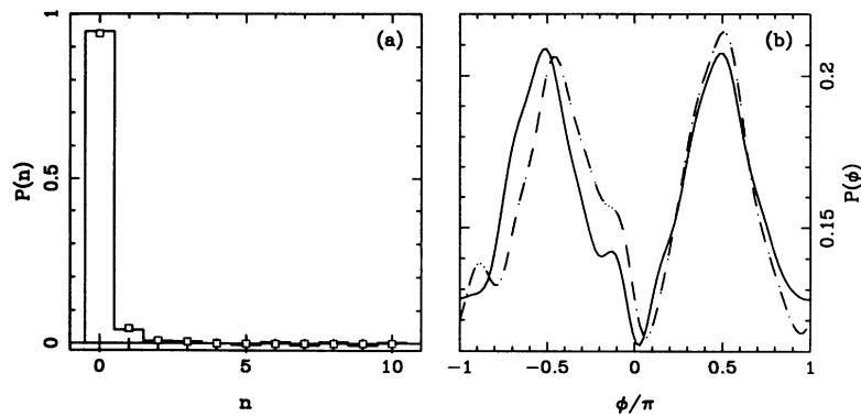
FIG. 5. Tomographic reconstruction from homodyne experimental data kindly provided by Beck and Raymer. Data have been grouped into 40 subensembles of 100 points for each of the F = 27 scanning phases. (a) Number probability distribution as in Fig. 4: the small squares correspond to evaluations provided by Beck and Raymer according to the original reconstruction method of Ref. [1]. (b) Ideal phase probability distribution: the full line is from the present method and the dashed line is from Beck and Raymer (see also Ref. [2]).
