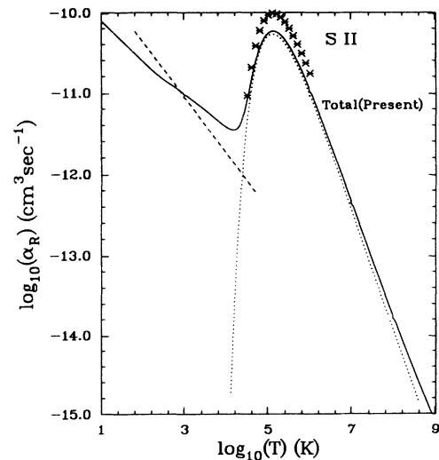
FIG. 9. Recombination rate coefficients for \text{S III} + e \rightarrow \text{S II} . The solid curve represents the present total rate coefficient. Comparison is made with RR rate coefficients (dashed curve) of Ref. [24], high- T DR rate coefficients of Ref. [25] (dotted curve) and of Ref. [26] (asterisks).
