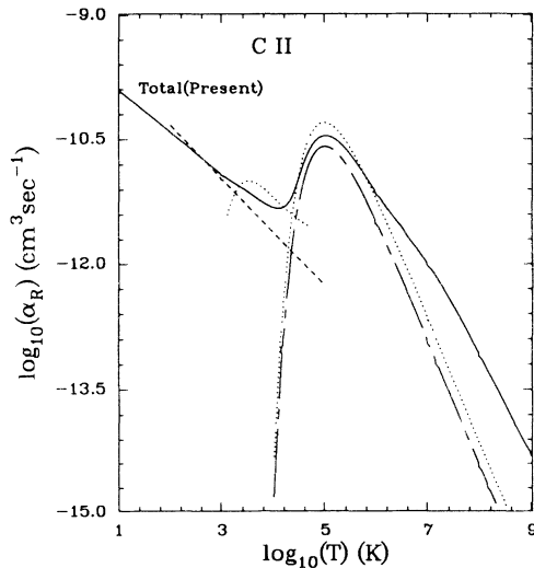
FIG. 8. Recombination rate coefficients for \text{C III} + e \rightarrow \text{C II} . The solid curve represents the present total rate coefficient and the dashed-chain curve represents the high- n contribution alone. Comparison is made with RR rate coefficients (dashed curve) of Ref. [24], low- T DR rate coefficients (dotted curve) of Ref. [2], and high- T DR rate coefficients (dotted curve) of Ref. [25].
