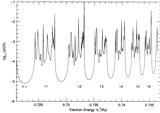
FIG. 4. Detailed DR collision strength. The resonances correspond to autoionizing states within the given n complexes. The example is for e + \text{S III} \rightarrow \text{S II} where the resonances converge onto the excited S III state 3s3p^3(^3D^o) , and the emitted photon spectrum shown is due to radiative transition to the ground state 3s^23p^2(^3P) .
