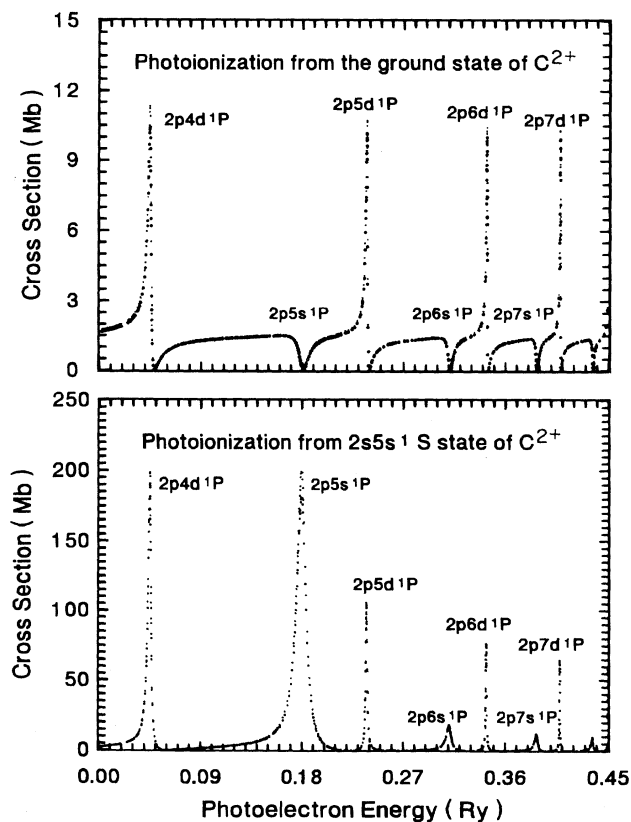
FIG. 1. Photoionization cross sections from the 2s^2\ ^1S ground state and the 2s5s\ ^1S bound excited state of the Be-like C^{2+} ion.
