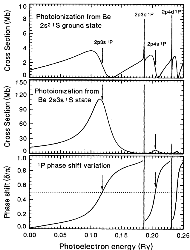
FIG. 2. Photoionization cross sections from the 2s^2\ ^1S ground state and the 2s3s\ ^1S bound excited state of the Be atom. The background scattering phase shifts are subtracted so that the resonant energy can be identified at a phase shift \delta = \pi/2 .
