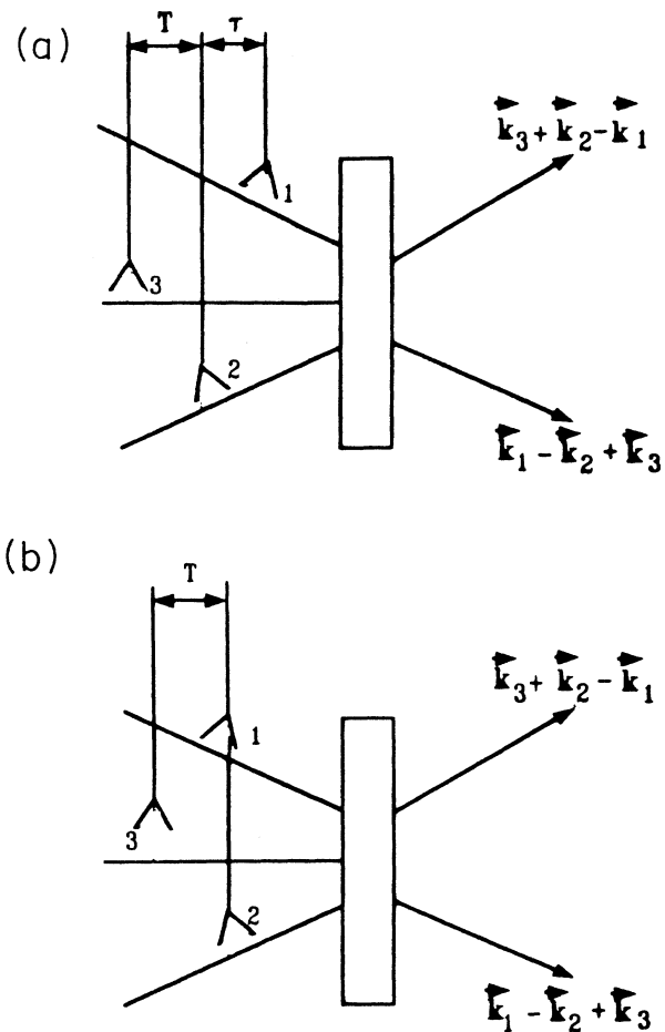
FIG. 1. Geometry for three-pulse time-delayed four-wave-mixing experiments: (a) grating on the basis of a polarization ( \tau variable, T = \text{const} ); (b) population grating ( \tau = 0 , T variable).
