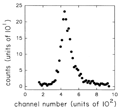
FIG. 2. Spectrum of coincidence counts as a function of time delay between the photodiode and the microchannel-plate signals. Each channel corresponds to a delay of 19.5 ns, and the data shown were binned in 15-channel increments.
