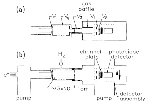
FIG. 1. Schematic diagram of the experiment: (a) top view showing the beam-switching grid V_1 , gas-cell electrode V_g , repelling electrode V_3 , and the retarding grids V_4 and V_5 ; (b) side view showing the structure of the gas cell and detector.
