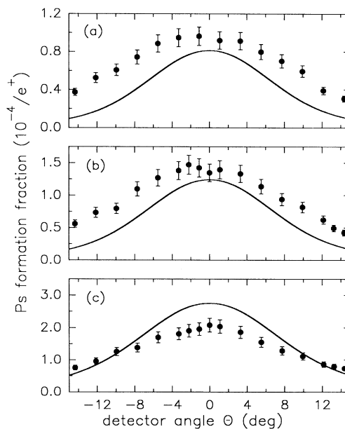
FIG. 3. The positronium formation fraction as a function of detector angle \theta for positron energies of (a) 100 eV, (b) 80 eV, and (c) 50 eV. The angle \theta is defined as that between the incident positron beam direction and the line between the center of the gas cell and the center of the detector aperture. The experimental values (solid circles) are compared with the theoretical predictions (solid lines) from Ref. [10].
