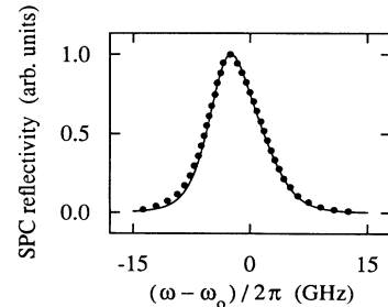
FIG. 6. SPC reflectivity from Fig. 5, for a number density of N = 1.5 \times 10^{17} \text{ cm}^{-3} . The solid circles are the measured values and the line is the corresponding theoretical prediction.
