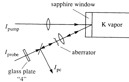
FIG. 3. Schematic of the experimental setup used to demonstrate aberration correction and to measure the SPC signal (without the aberrator and glass plate).
