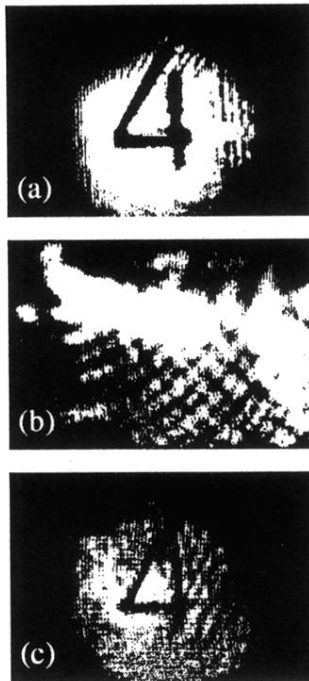
FIG. 4. (a) Image-bearing beam. (b) Image-bearing beam after retracting the aberrator due to reflection by an ordinary mirror. (c) Image-bearing beam after retracting the aberrator due to reflection by a SPC mirror. In (c), the wave-front reversal of the SPC mirror causes the aberration seen in (b) to be removed.
