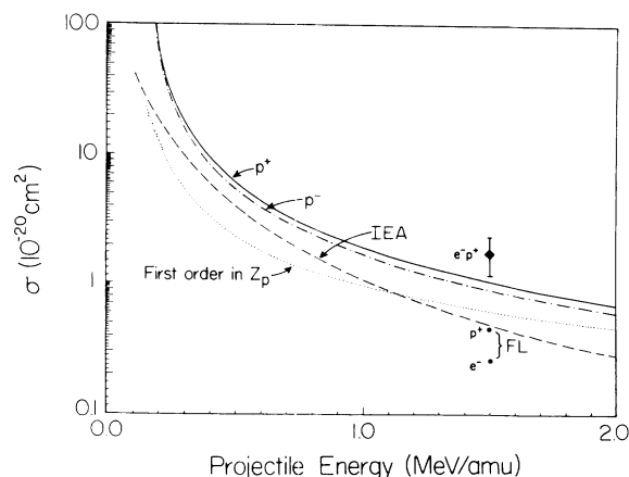
FIG. 1. Excitation of helium into the 2p^2\ ^1D^e final state. The solid curve is the second-order theory for proton impact and the dash-dotted curve is for antiprotons. The dashed curve is the independent-electron approximation and the dotted curve is the first-order result. The data points for proton and electron impact are from Giese et al. (Ref. [13]) and the other two points at 1.5 MeV/amu are the close-coupling calculation of Fritsch and Lin (Ref. [15]).
