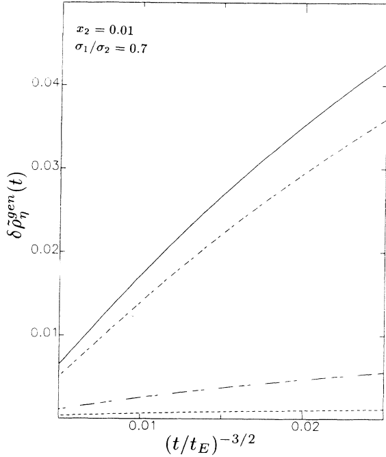
FIG. 3. The three contributions to \delta\tilde{\rho}_\eta^{gen}(t) from the coupling of different pairs of modes, ++ (dashed line), -- (long-short dash), and +- (long-short-short dash), are shown separately as functions of (t/t_E)^{-3/2} for x_2=0.01 and \sigma_1/\sigma_2=0.7 . The total correlation function is also shown (solid line).
