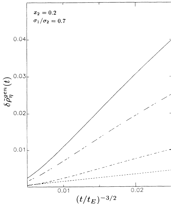
FIG. 4. Same as Fig. 3 for x_2=0.2 .
