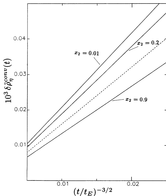
FIG. 1. The conventional mode-coupling contribution to the STAF 10^3 \delta\rho_\eta^{\text{conv}}(t) as a function of (t/t_E)^{-3/2} for \sigma_1/\sigma_2 = 0.7 and three values of the concentration x_2 . The one-component fluid result is also shown (dashed line).
