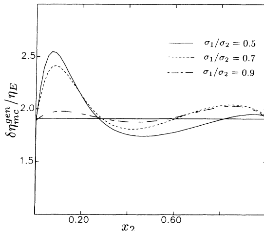
FIG. 8. The reduced generalized mode-coupling shear viscosity \delta\eta_{\text{mc}}^{\text{gen}}/\eta_E as a function of x_2 for various values of the size ratio: \sigma_1/\sigma_2=0.5 (solid line), \sigma_1/\sigma_2=0.7 (dashed line), and \sigma_1/\sigma_2=0.9 (long-short dash). The value of \delta\eta_{\text{mc}}^{\text{gen}}/\eta_E for a one-component fluid is also shown.
