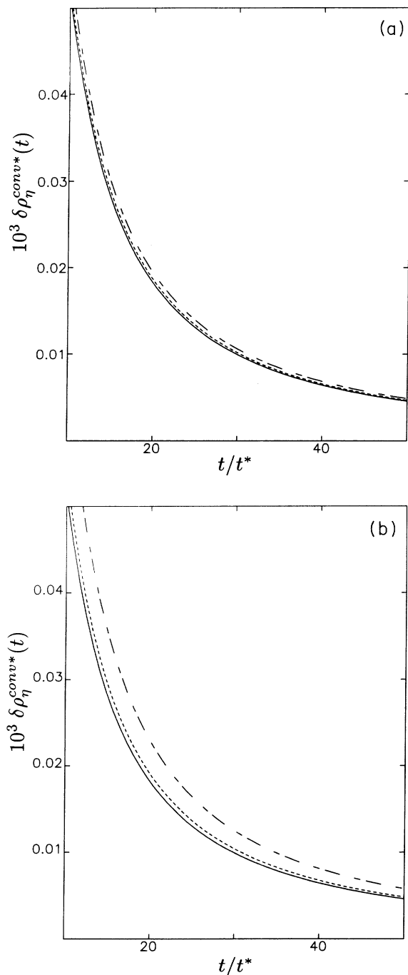
FIG. 6. The conventional mode-coupling contribution to the STAF, 10^3\delta\rho_\eta^{\text{conv}*}(t) , as a function of t/t^* for \sigma_1/\sigma_2=0.7 and various values of the concentration: (a) x_2=0.01 (solid line), x_2=0.1 (dashed line), and x_2=0.2 (long-short dash); (b) x_2=0.9 (solid line), x_2=0.6 (dashed line), and x_2=0.4 (long-short dash).
