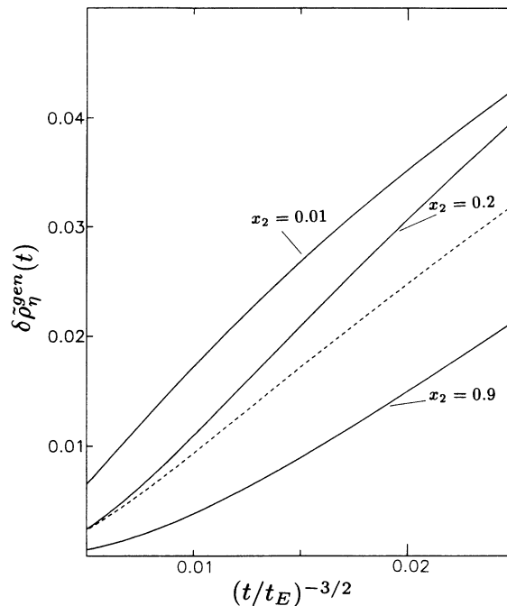
FIG. 2. The generalized mode-coupling contribution to the STAF \delta\rho_\eta^{\text{gen}}(t) as a function of (t/t_E)^{-3/2} for \sigma_1/\sigma_2 = 0.7 and three values of the concentration x_2 . The one-component fluid results is also shown (dashed line).
