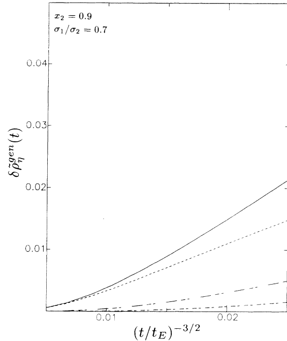
FIG. 5. Same as Fig. 3 for x_2=0.9 .
